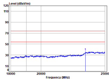
Car 2.4G_SRD_TX_CH_M_Horizontal
