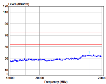
Car 2.4G_SRD_TX_CH_M_Vertical
