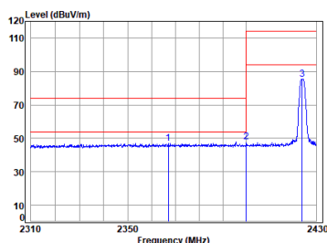
Remote 2.4G SRD_TX_CH_L_Vertical
