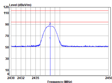
Remote 2.4G SRD_TX_CH_M_Vertical
