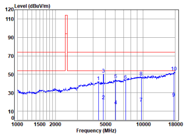
2.4G_SRD_LOW_TX_Vertical
