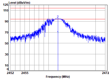
2.4G_SRD_HIGH_TX_Horizontal
