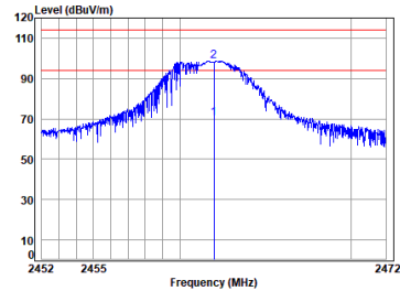
2.4G_SRD_HIGH_TX_Vertical
