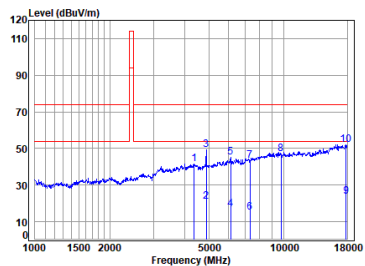
2.4G_SRD_MID_TX_Vertical
