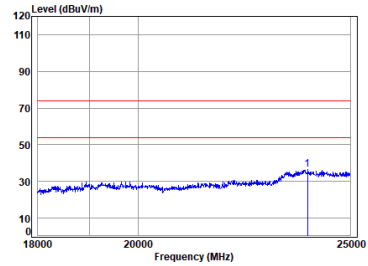
2.4G_SRD_HIGH_TX_Vertical
