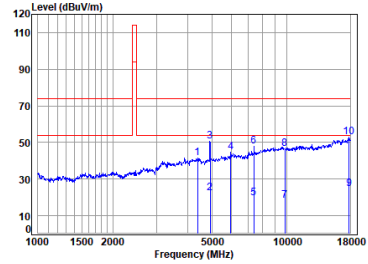
2.4G_SRD_HIGH_TX_Vertical
