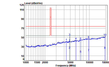
2.4G_SRD_MID_TX_Horizontal
