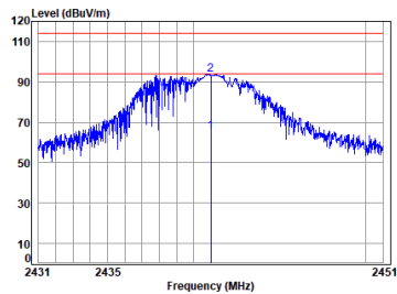
2.4G_SRD_MID_TX_Horizontal
