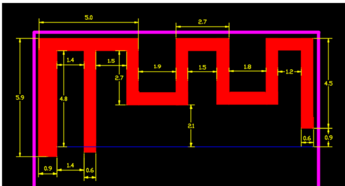
Antenna Dimensions
