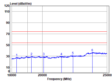
2.4G_TX_CH_M_Vertical
