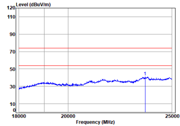
2.4G_SRD_TX_HIGH_Vertical
