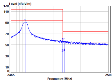
2.4G_SRD_TX_HIGH_Vertical
