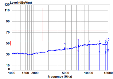
2.4G_SRD_TX_HIGH_Vertical
