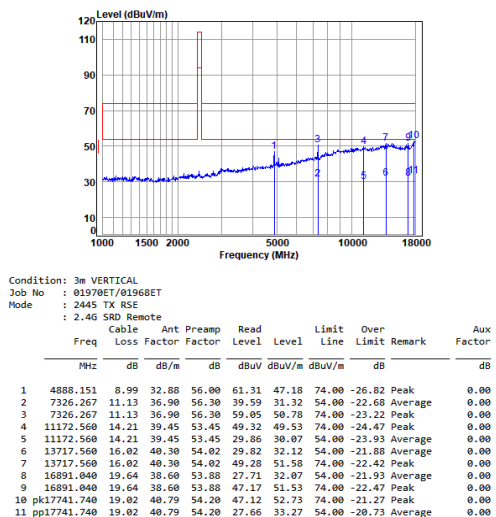
2.4G_SRD_TX_MID_Vertical
