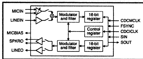
CODEC Block Diagram
