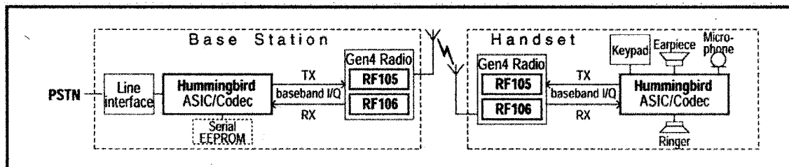
Spread Spectrum System Architecture
