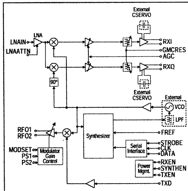
RF Block Diagram
