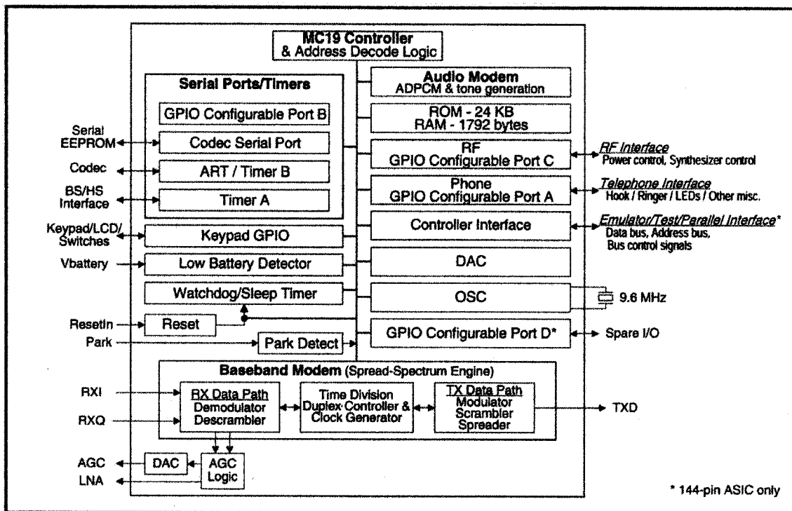
ASIC Block Diagram
