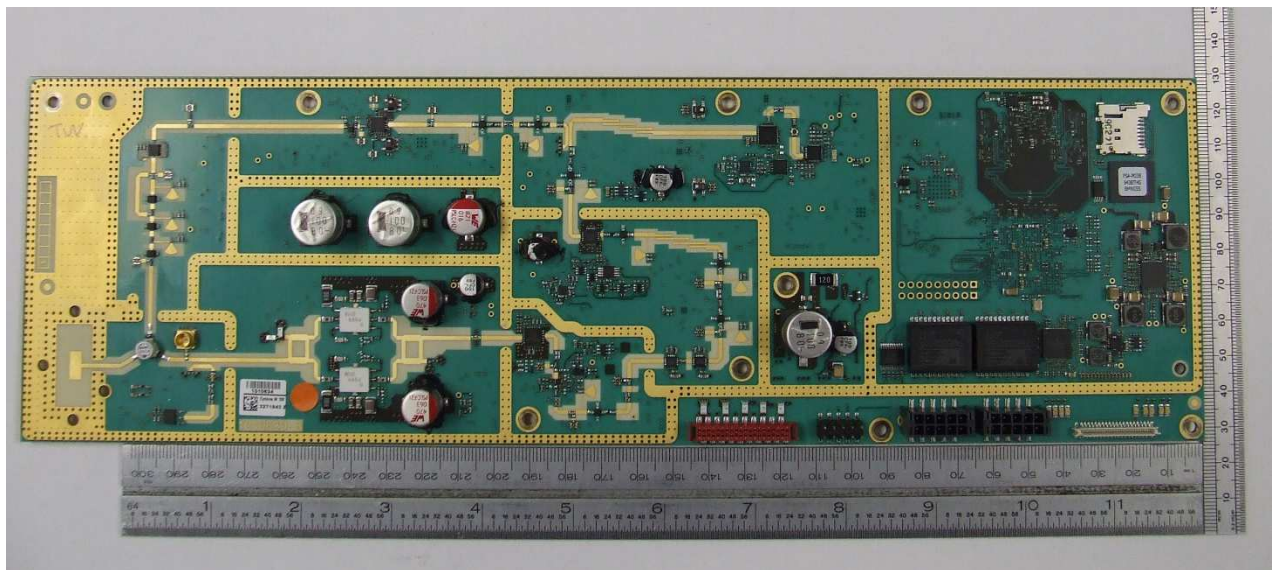
Figure 3 – Cyclone Pro Main (RF) PCB (top)
