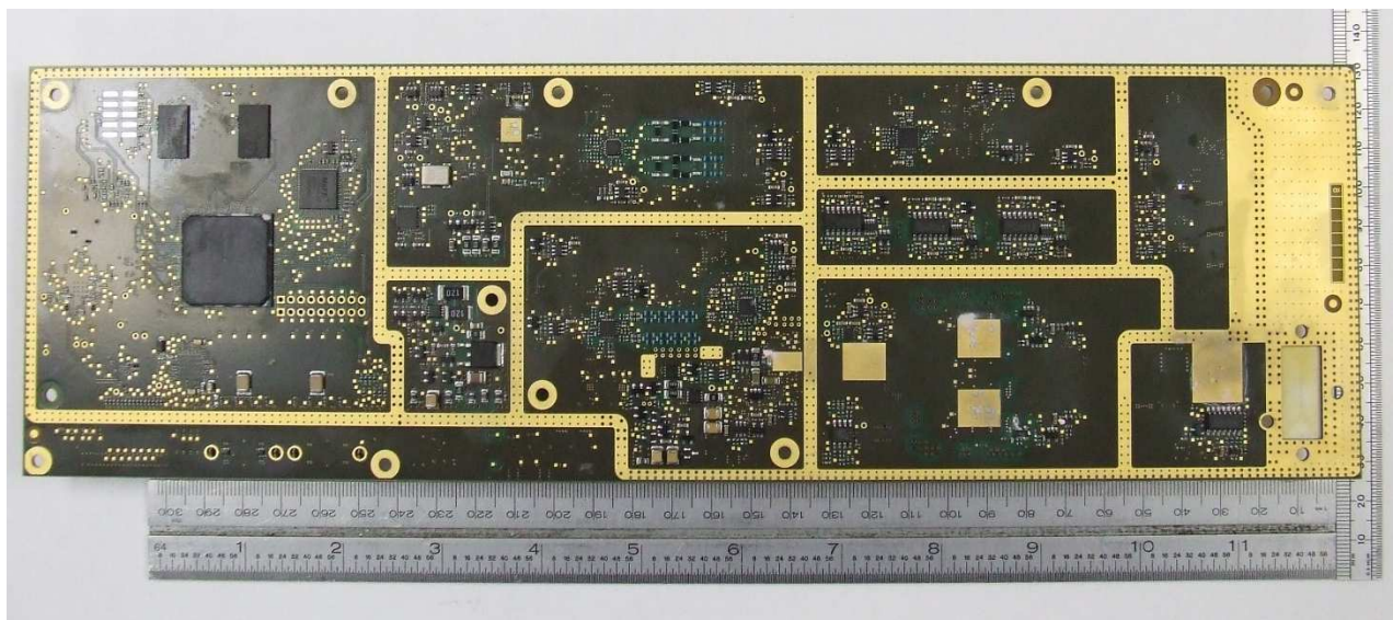
Figure 4 – Cyclone Pro Main (RF) PCB (bottom)
