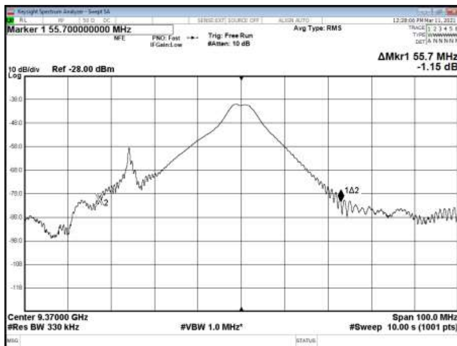
Figure 48 - 9370, FM, 750 ns, 40 dB Bandwidth
