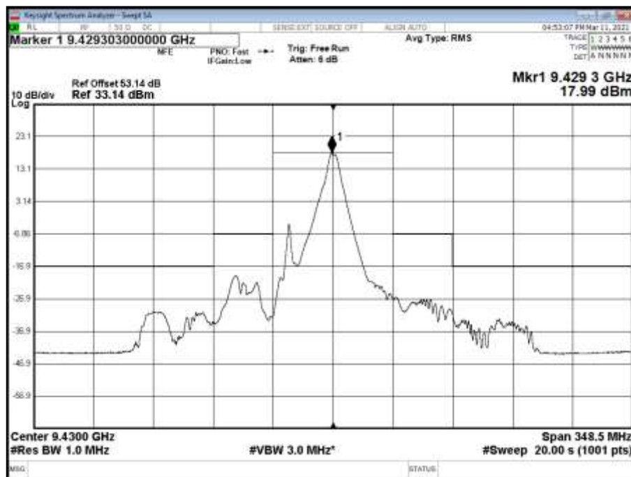
Figure 60 - 9430 MHz, FM, 750 ns (FCC Mask)
