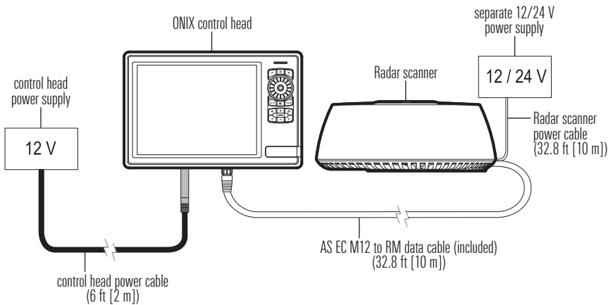
Example of a Schematic Diagram with a Direct Connection to the Control Head
