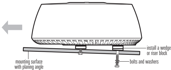
Mounting on an Angled Surface (or Planing Vessel)
