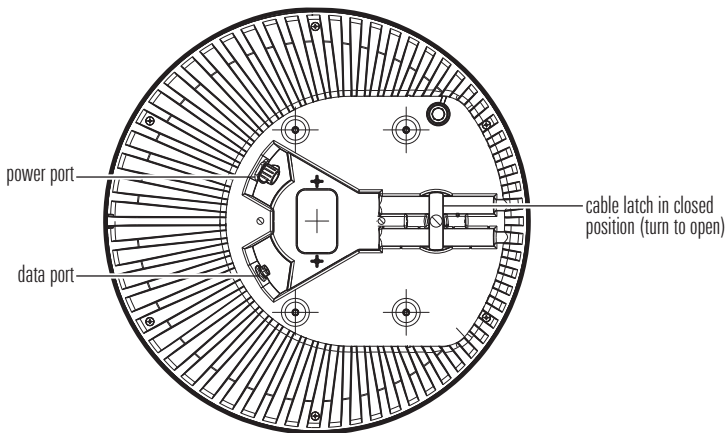
Locating the Cable Ports
