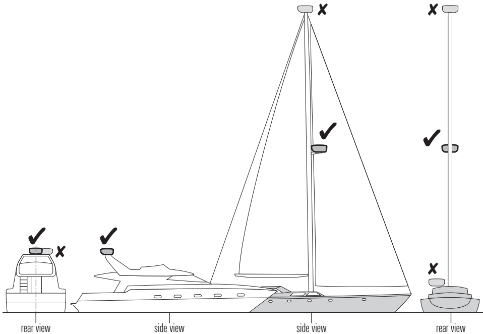
Determining the Mounting Location
