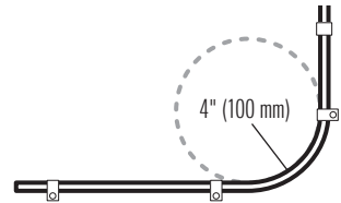
Avoiding Cable Bending
