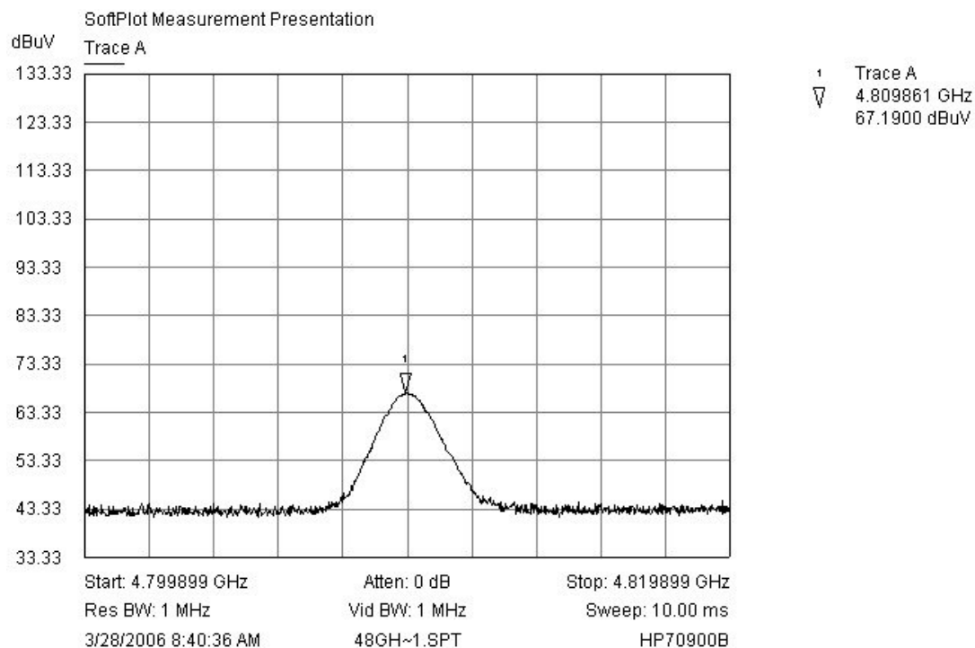
Figure 14 Channel 11 Vertical (Highest recorded 2 nd harmonic)
