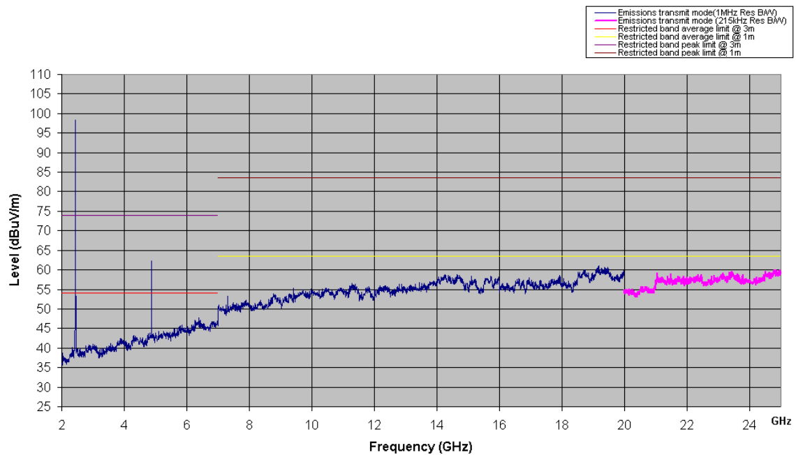
Figure 12 Composite graph of radiated emissions. EUT in Tx mode, channel 18
