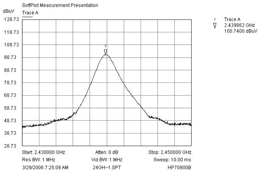
Figure 13 Channel 18 Vertical (Highest recorded fundamental frequency)
