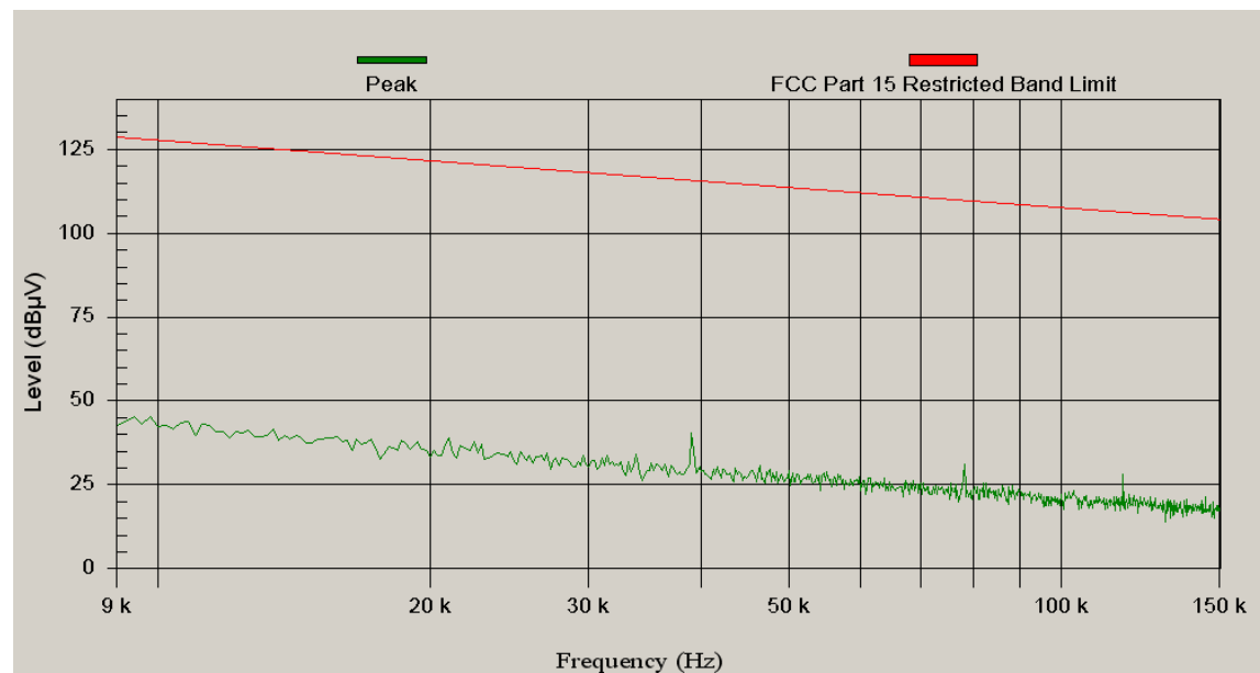
Figure 5 Composite graph of radiated emissions, antenna edge on from EUT
