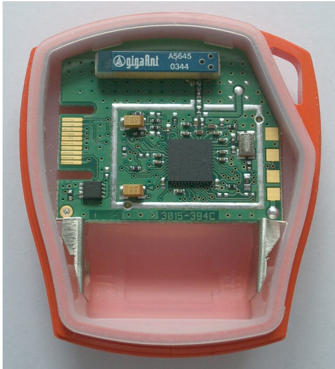
LifeTag Rear cover removed showing PCB and battery compartment
