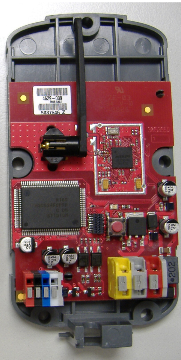
LT Base Station Front View, Primary and Secondary Covers Removed
