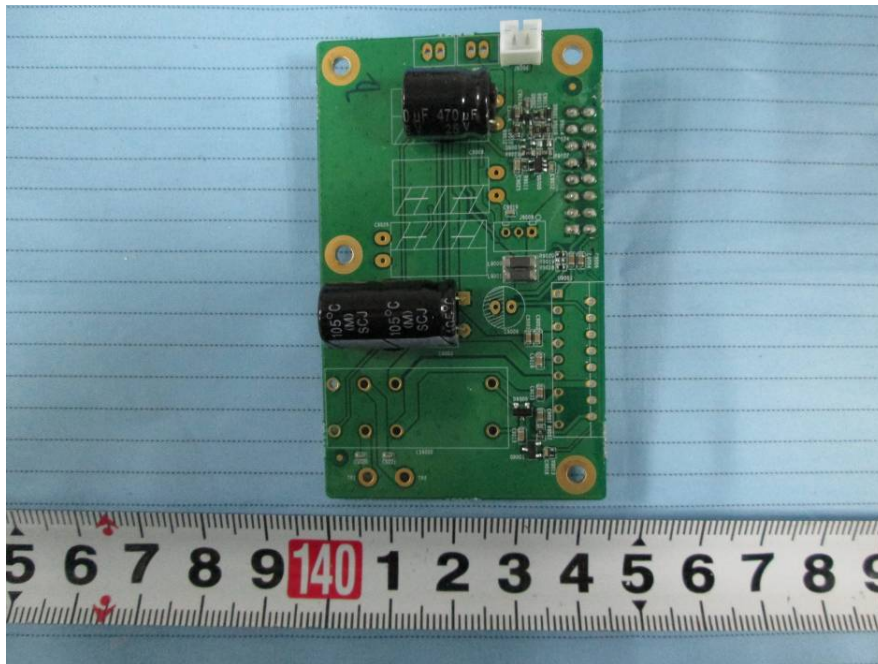
EUT –The Connect Board 2 Top View
