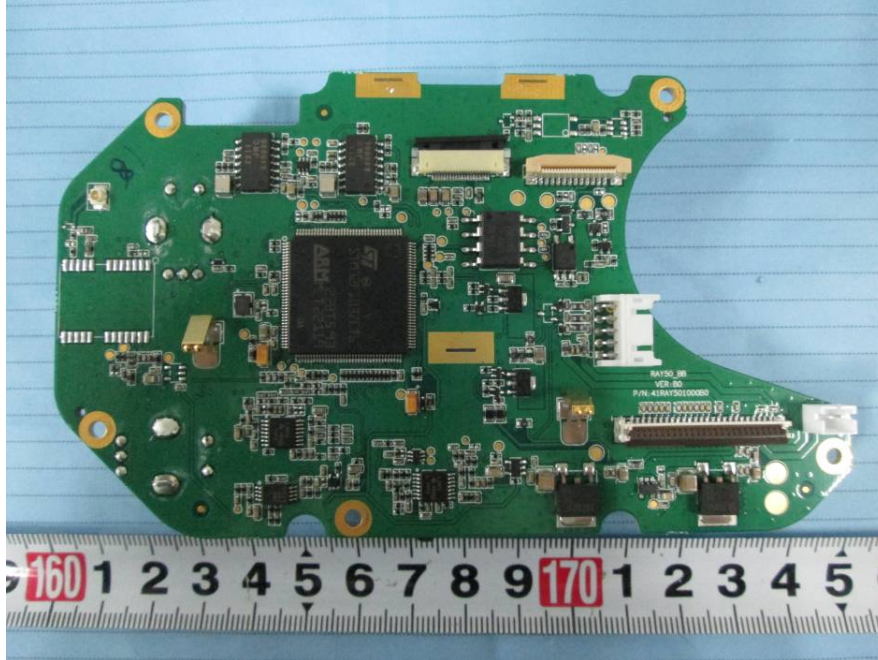
EUT –The Connect Board 1 Bottom View
