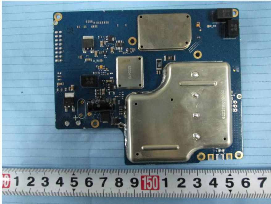
EUT –Base Main Board 1Top View 1
