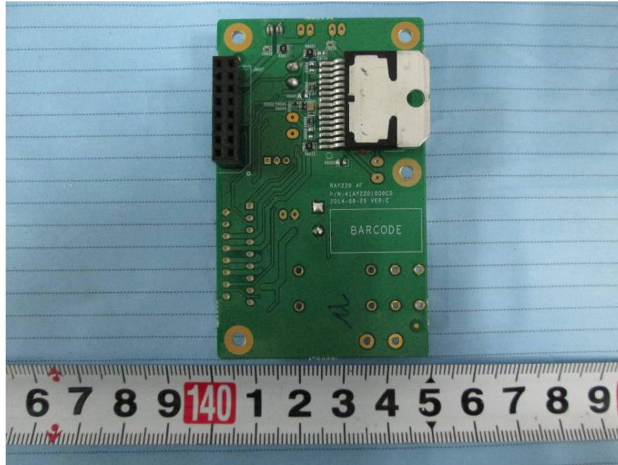
EUT –The Connect Board 2 Bottom View
