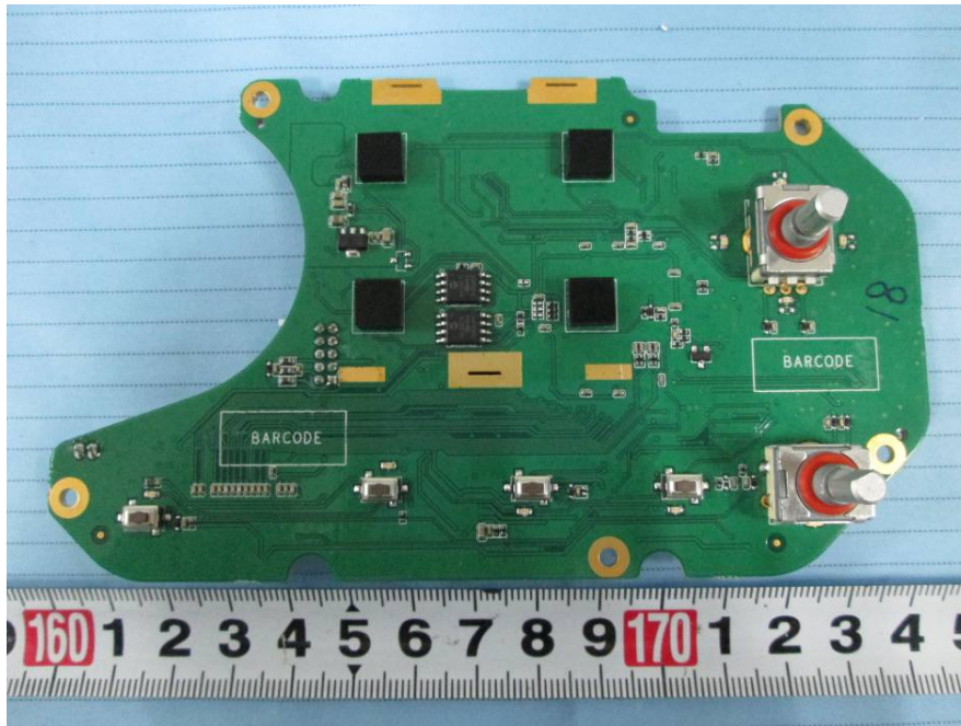
EUT –The Connect Board 1 Top View
