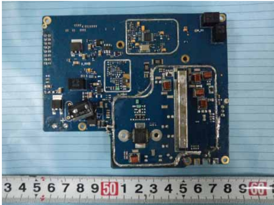
EUT –Base Main Board 1Top View 2
