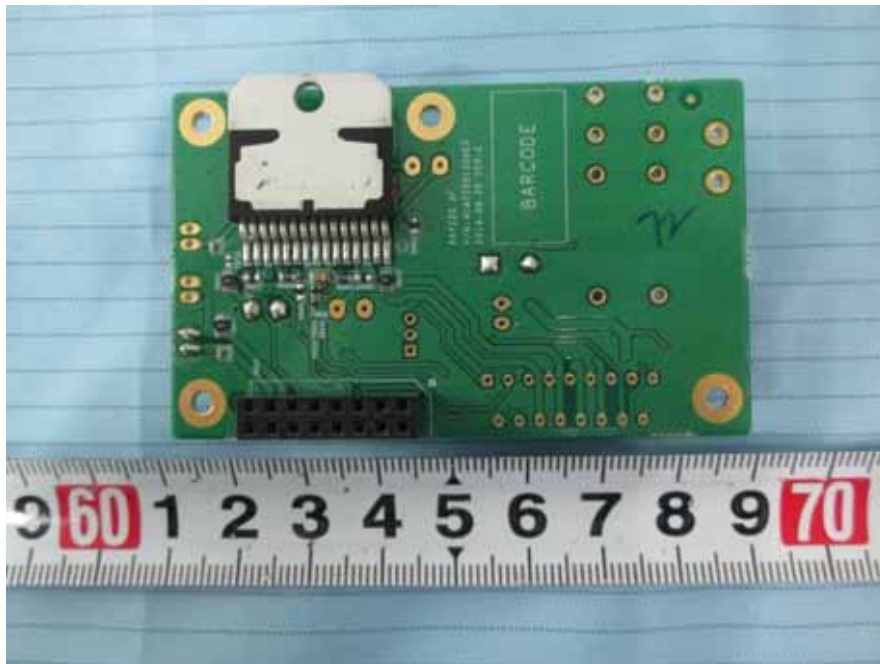
EUT –the connect board BottomView
