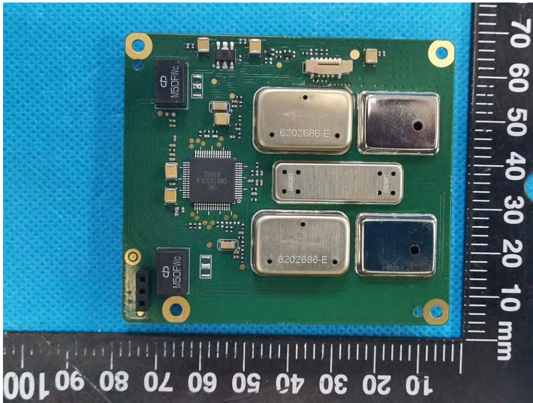
AIS Board
