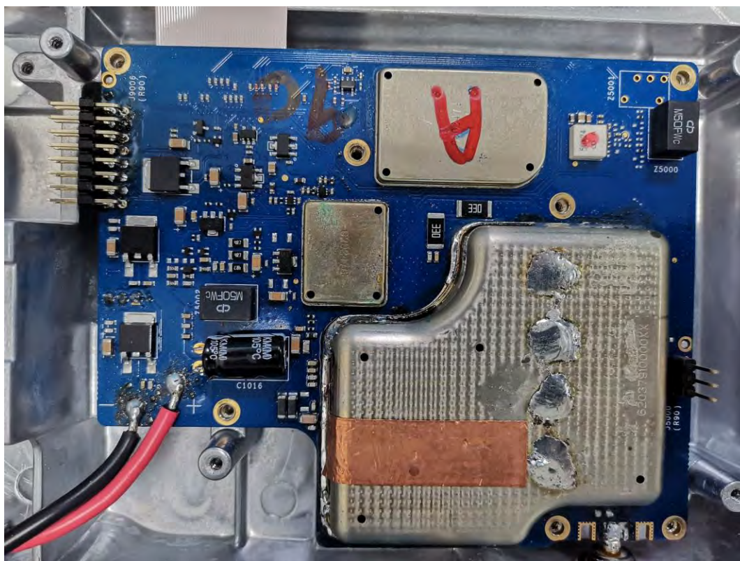
RF Board
