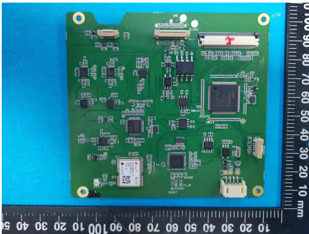
Main Board
