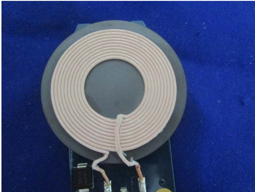
EUT – Wireless Charging Coil View
