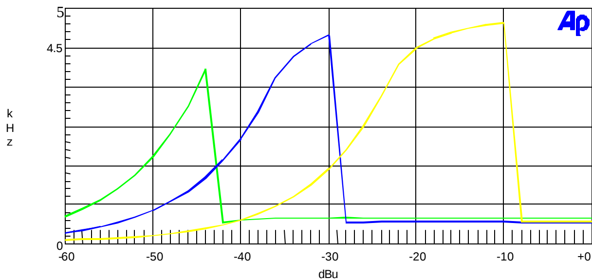
MODULATION LIMITING GRAPH 3.0KHz (Green), 1.0KHz (Blue), and 300Hz (Yellow)
