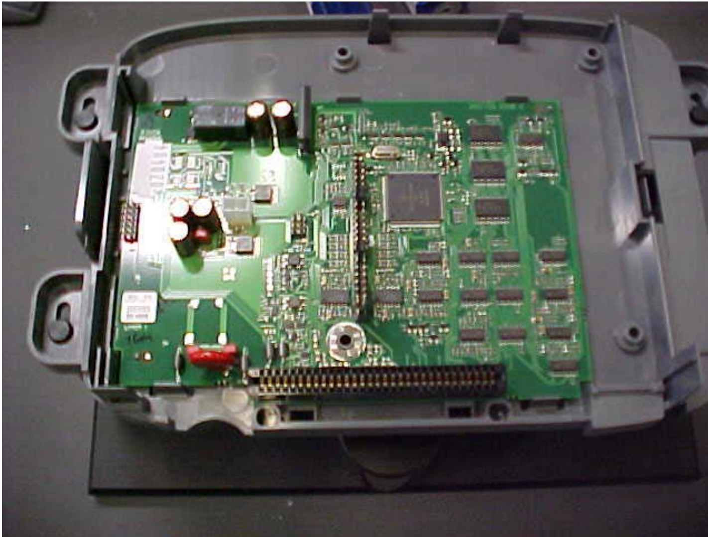
RAY 240 VHF Radio – Transceiver Unit
