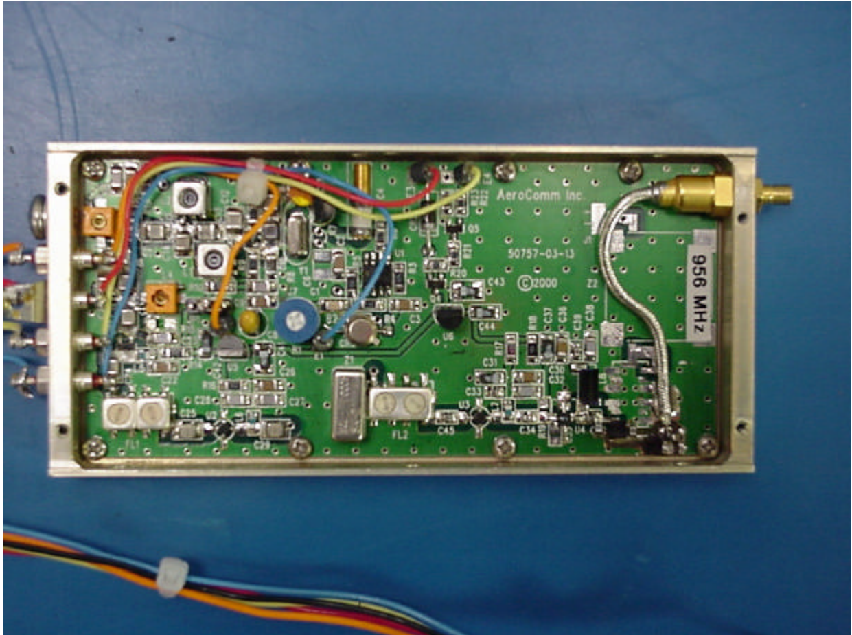
PHOTOGRAPH 7: COMPONENT SIDE
