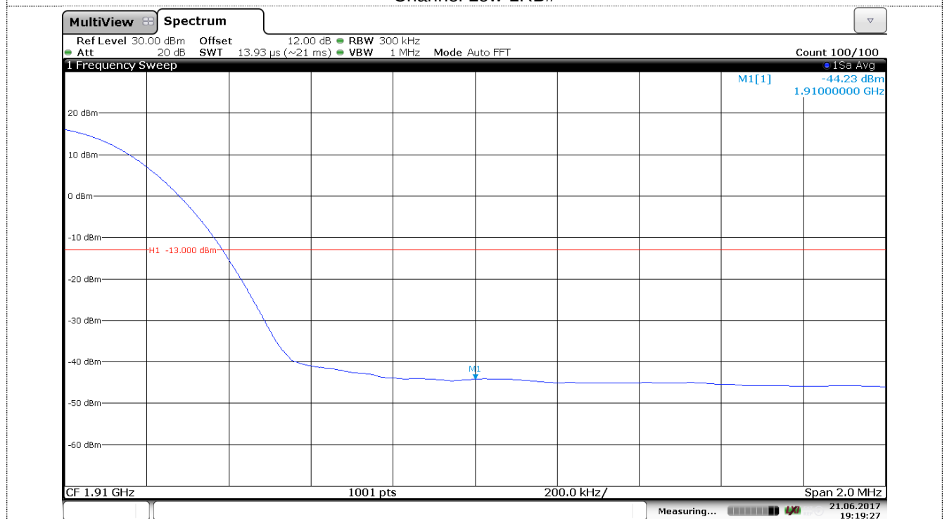
Channel High-1RB#
