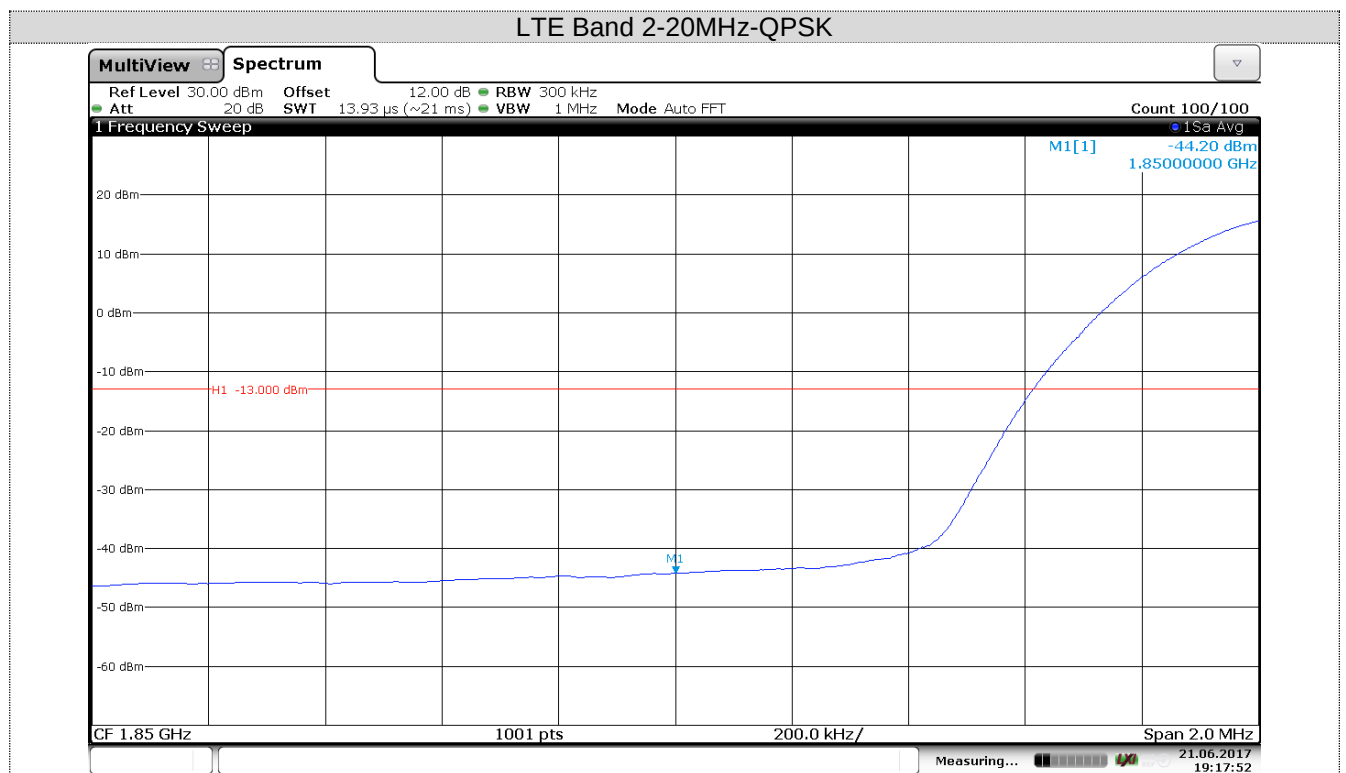
Channel Low-1RB#
