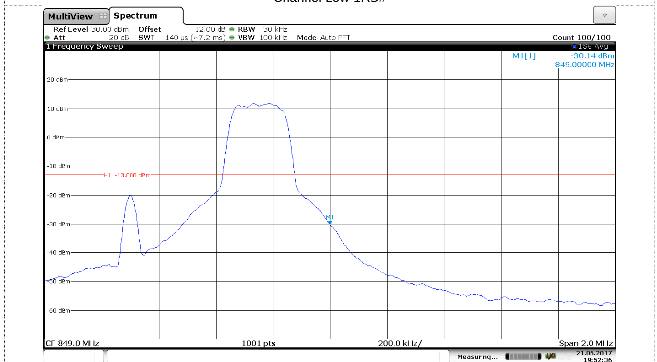
Channel High-1RB#
