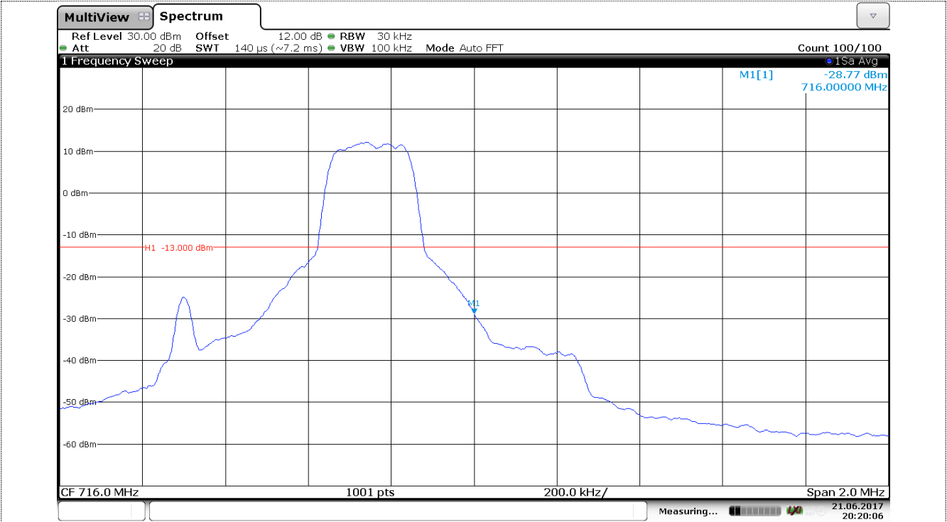
Channel Low-1RB#
