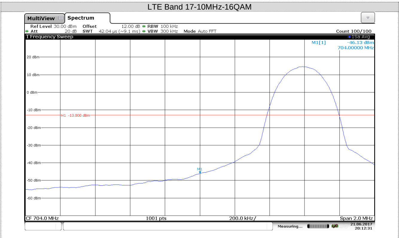
Channel Low-1RB#
