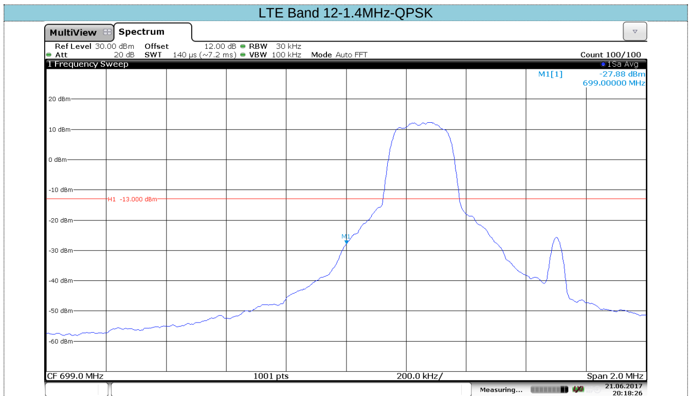
Channel Low-1RB#
