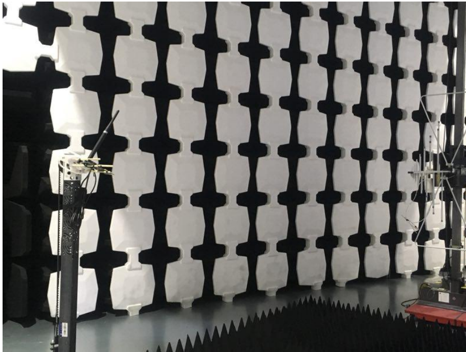
Description: Substitution Antenna for ERP Test
