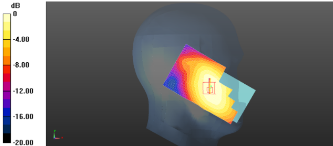
Left Head Cheek (LTE Band 17 Middle Channel)
