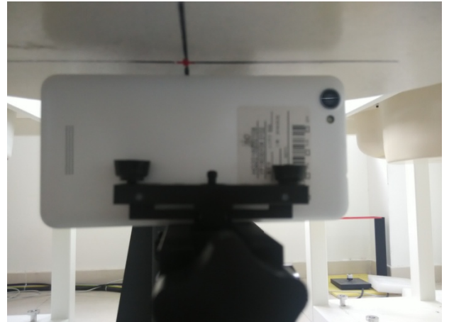
Hotspot mode - Right Side (10mm)
