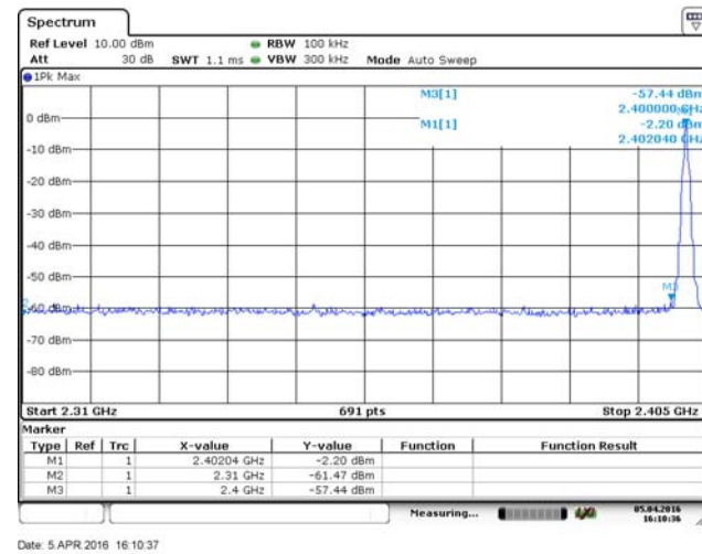
Bandedge- no hopping mode (CH00)
