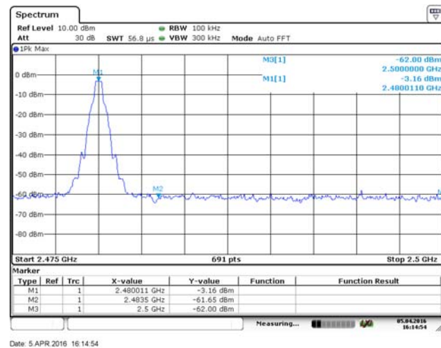
Bandedge- no hopping mode (CH78)
