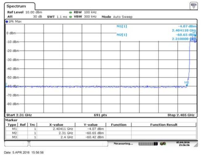
Bandedge- hopping mode (CH00)
