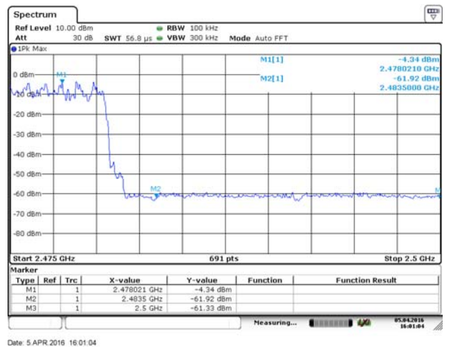
Bandedge- hopping mode (CH78)
