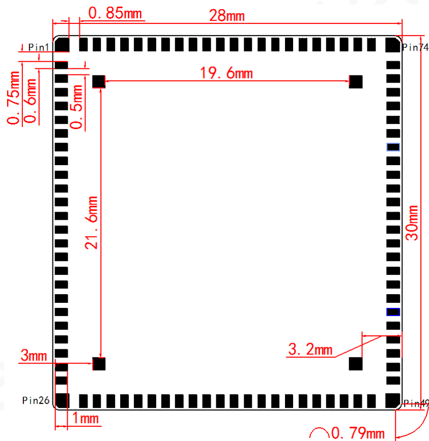
Figure 7-1 Bottom view
