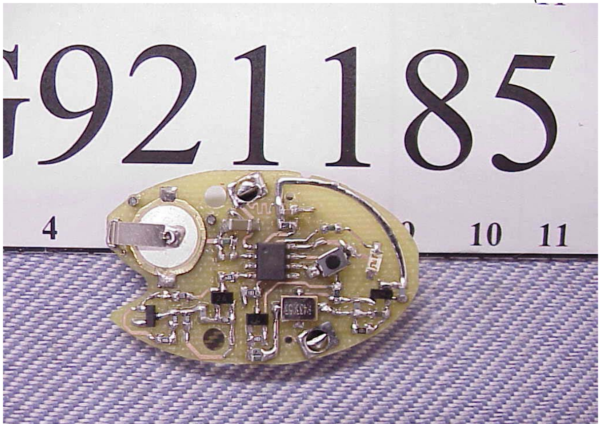
Photos 4 PCB View (Front Side)
