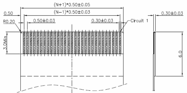
RECOMMENDED FFC/FFC DIMENSION
