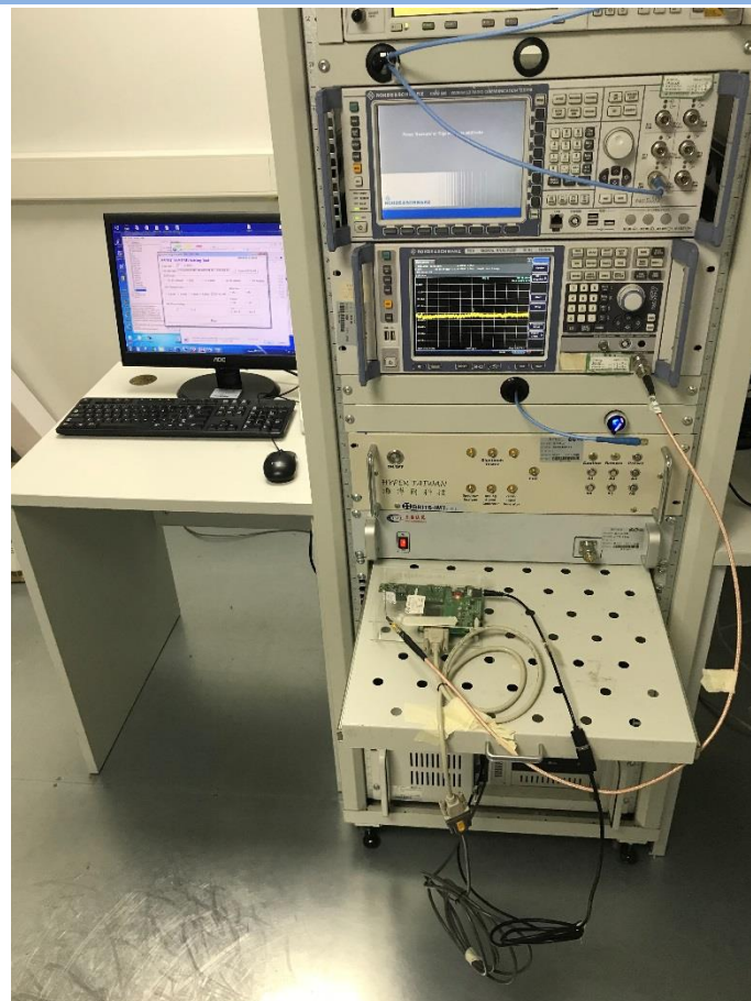
Conducted Test-5G WIFI
