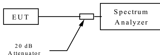
Figure 5 : Conducted spurious emission measurement configuration
