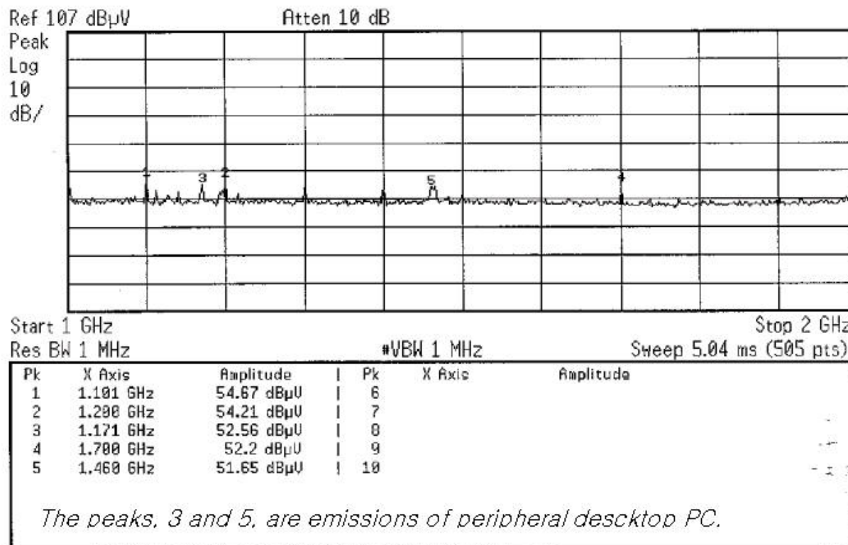
Emissions for above 1GHz
