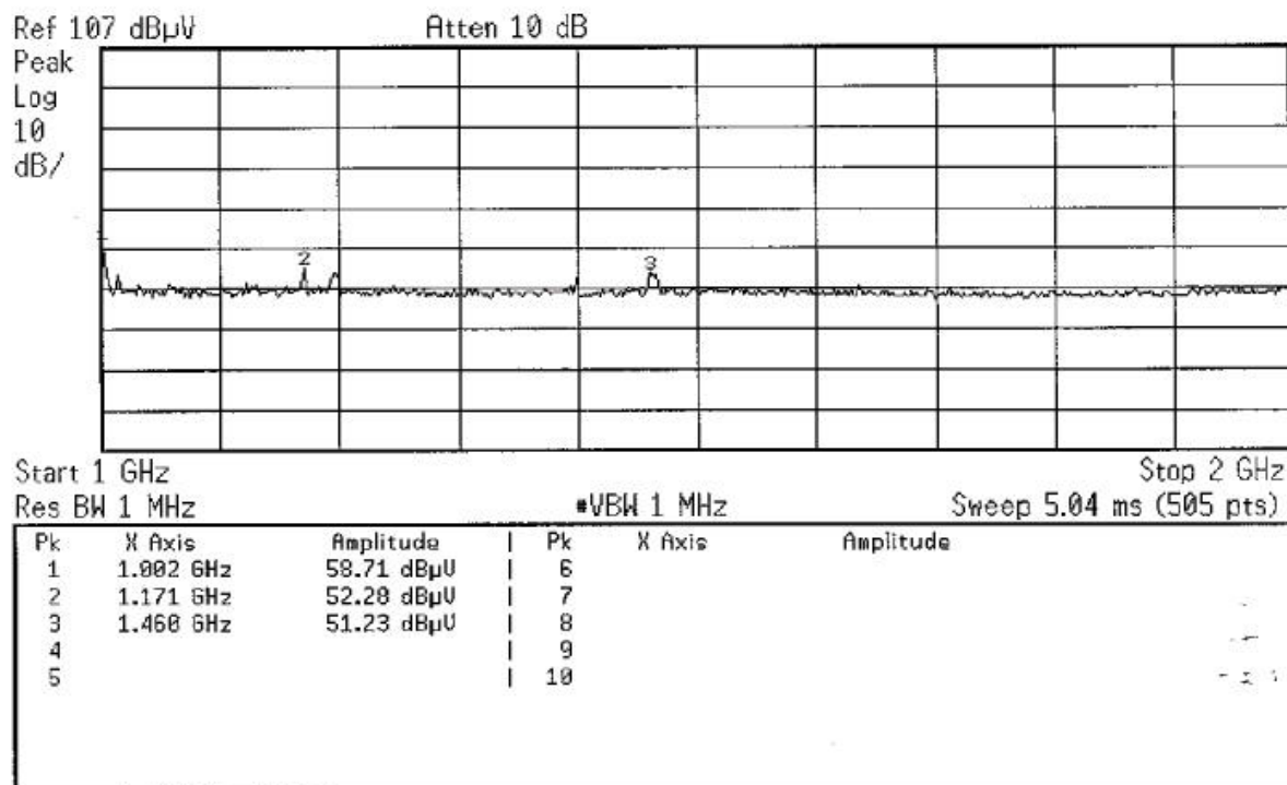
Emissions for Desktop PC above 1GHz
