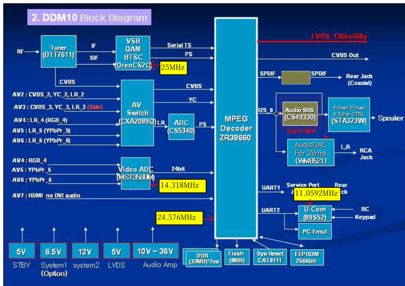
Fig. 3-1. DDM 10 Block Diagram
