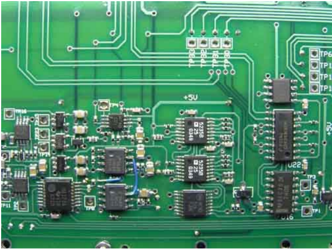
PCB RF Control Logic
