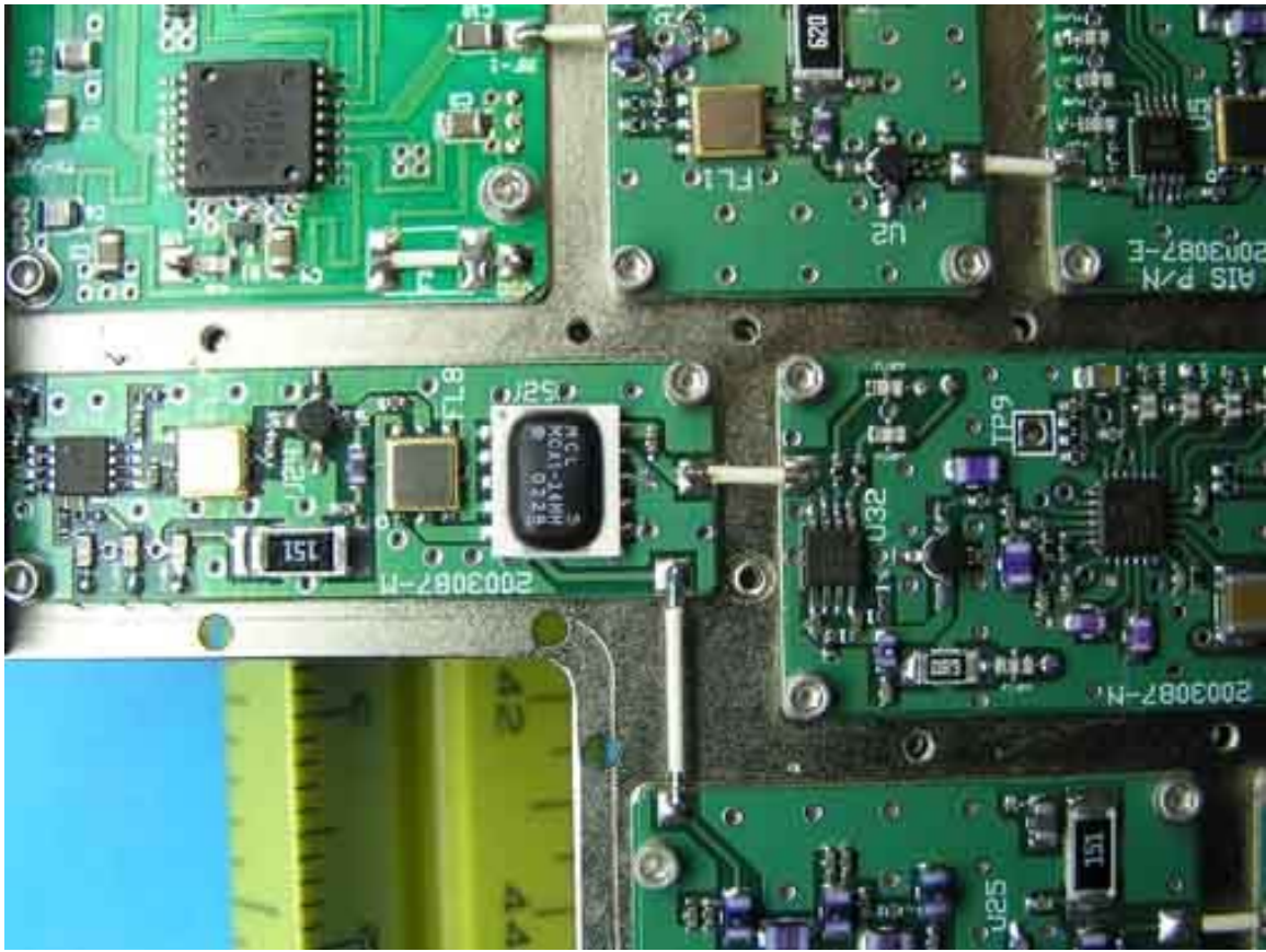
PCB RX Down Conv
