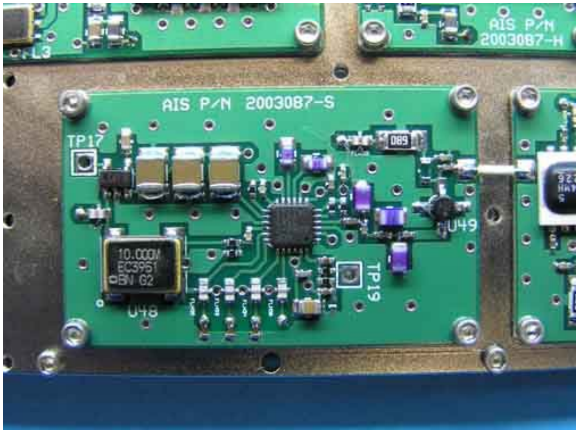
PCB TX Synthesizer
