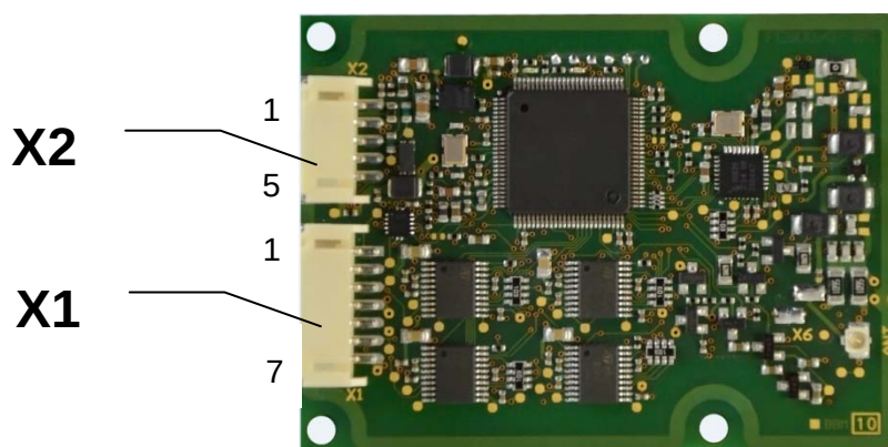
Figure 4: ID CPR74 - plug and connections
