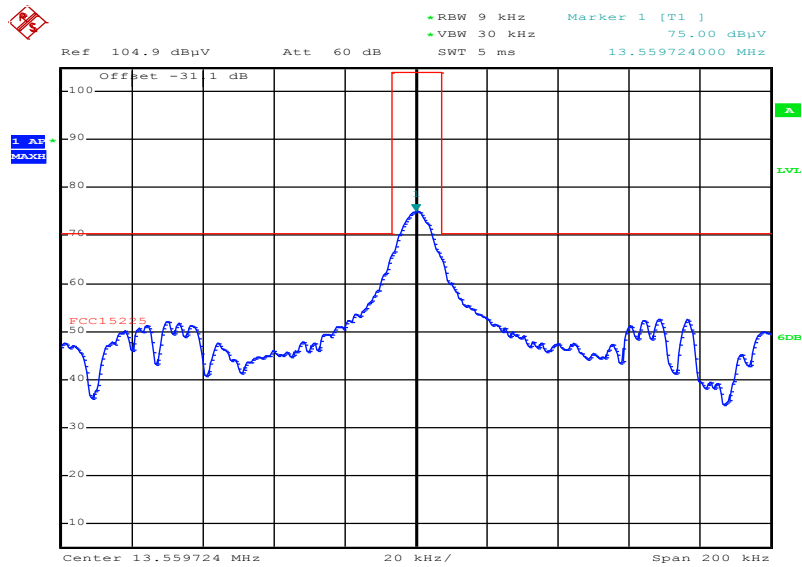
Plot 4: Spectrum mask (in detail)
