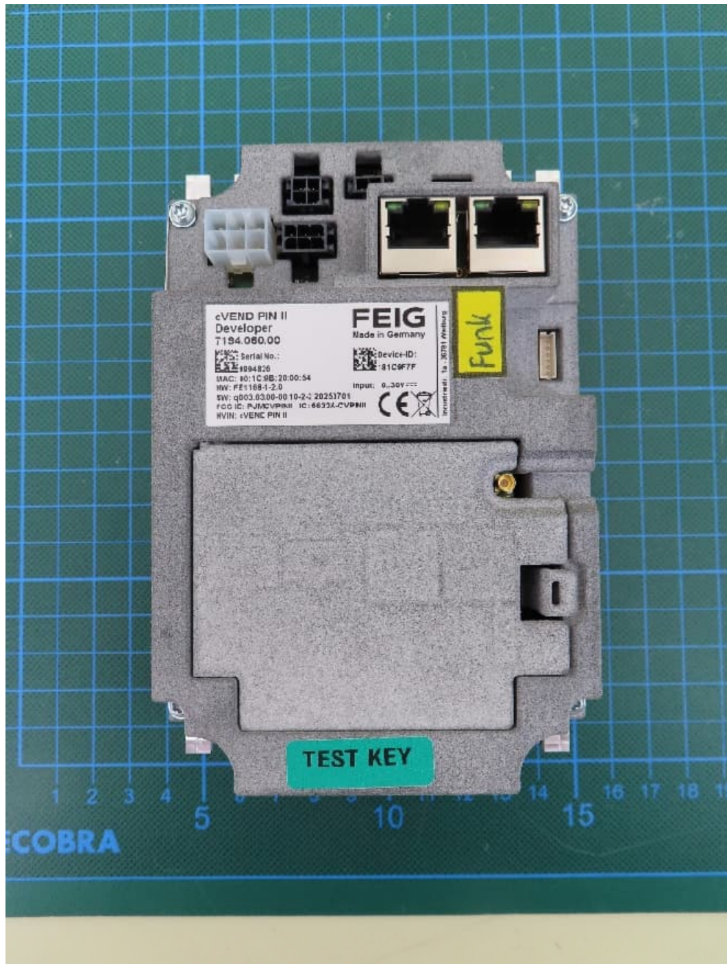
EUT, bottom view
