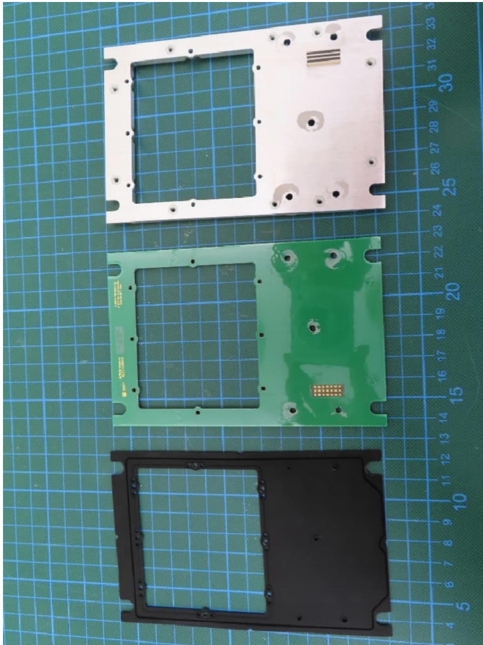
EUT, cVEND PIN II – Keyboard PCB, bottom view
