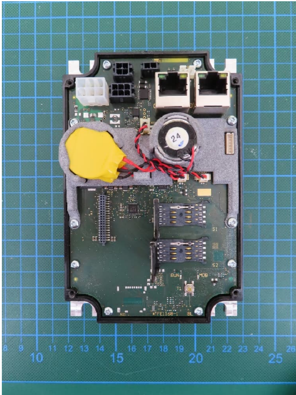
EUT, SAMs removed
