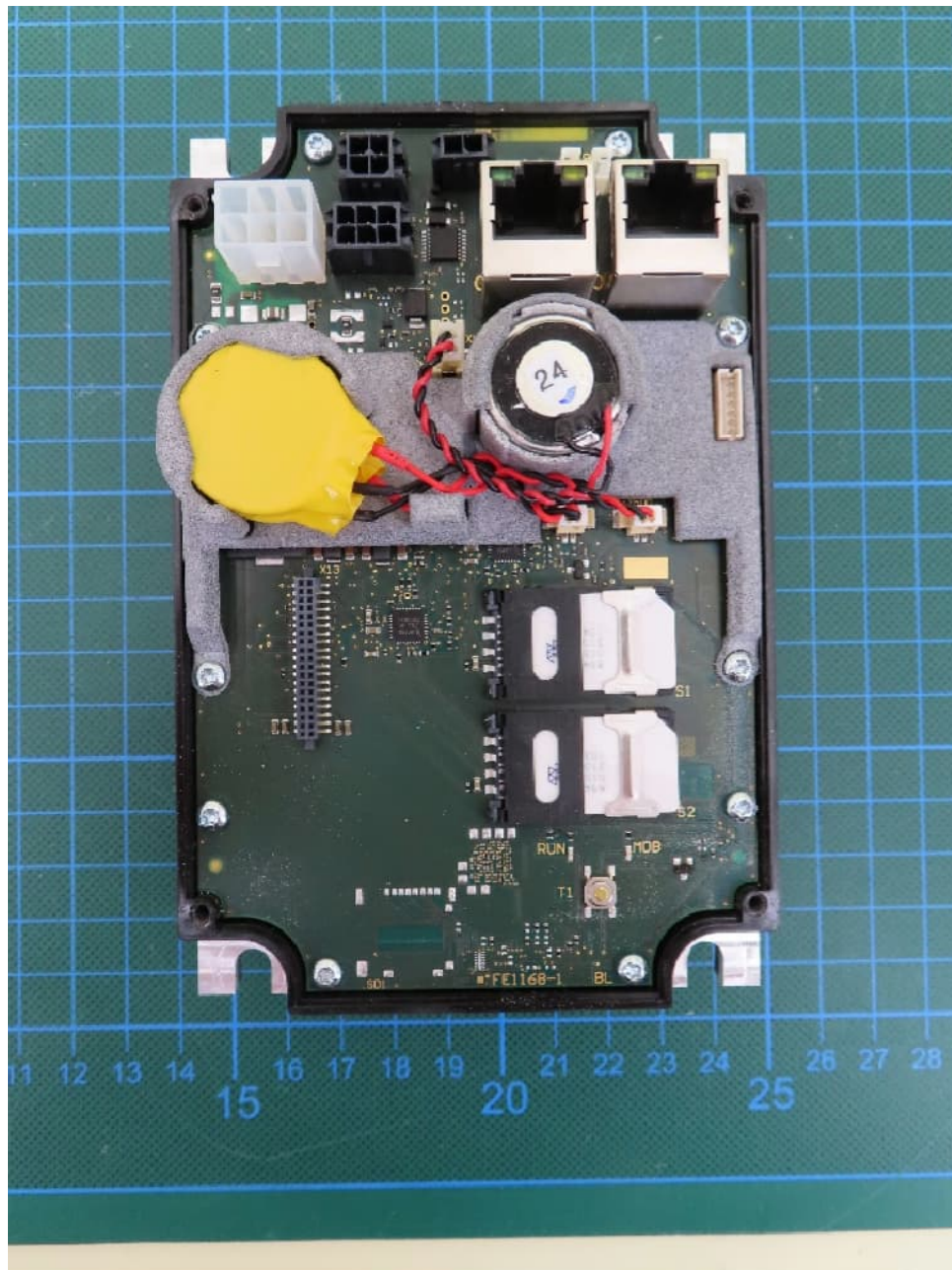
EUT, cover removed, view 2
