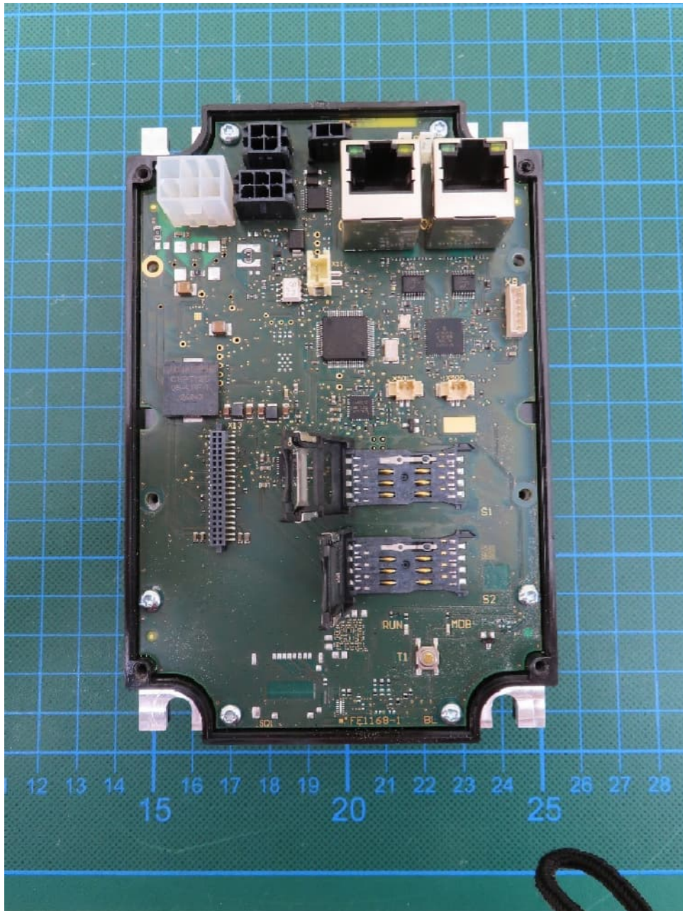
PCB PAY cVEND PIN II – Core, bottom view
