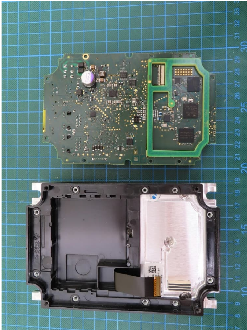
EUT, cVEND PIN II – Core removed
