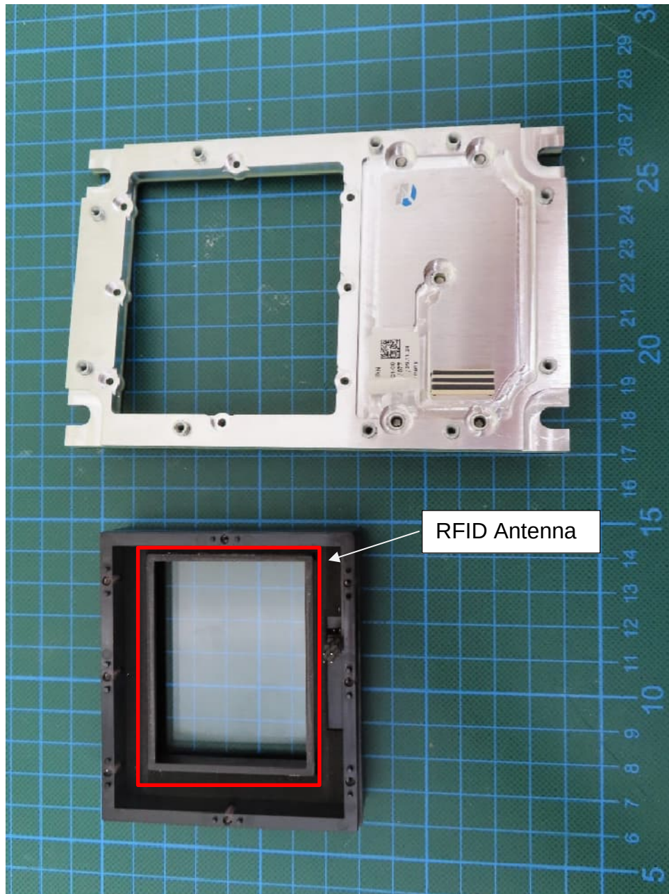
EUT, cVEND PIN II – Display cover with red marked Antenna removed
