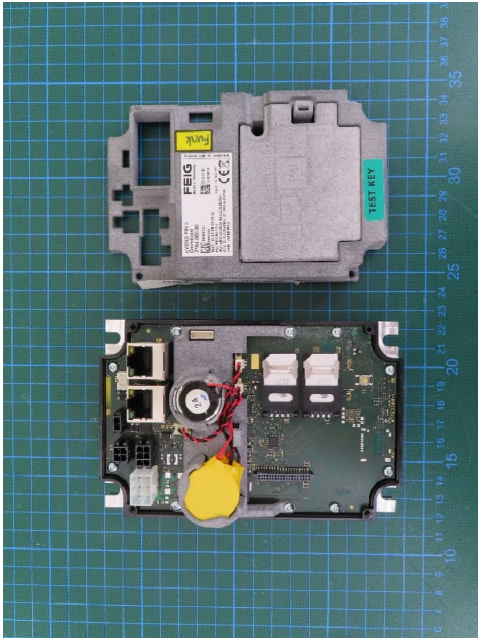
EUT, cover removed, view 1
