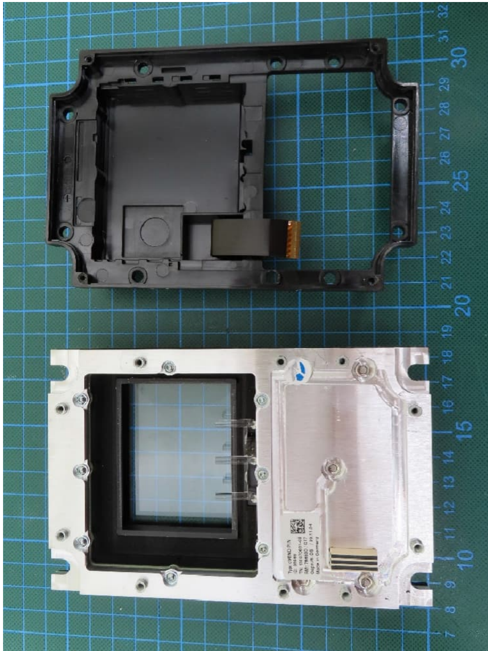
EUT cVEND PIN II – Display removed
