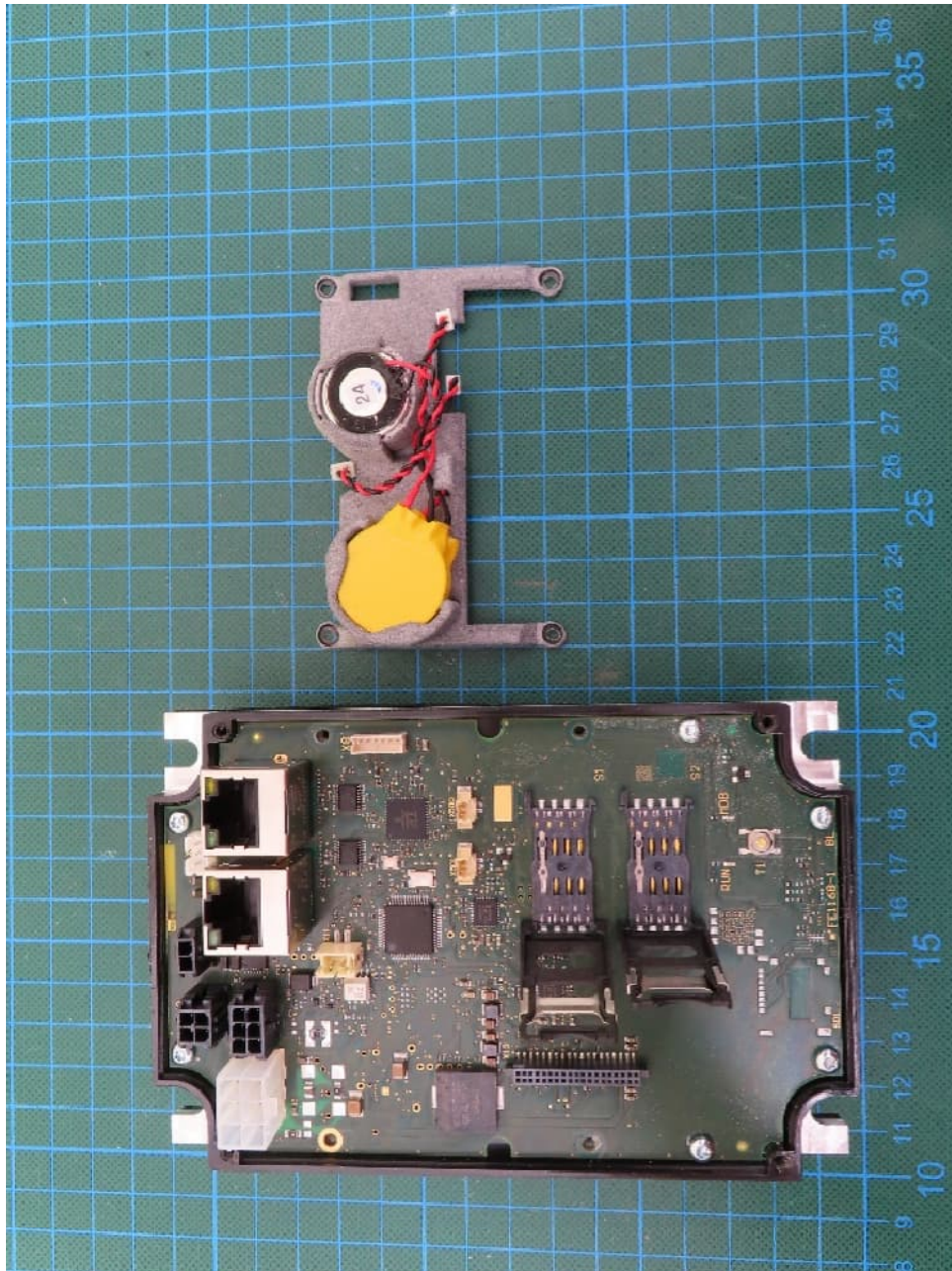
EUT, battery holder removed
