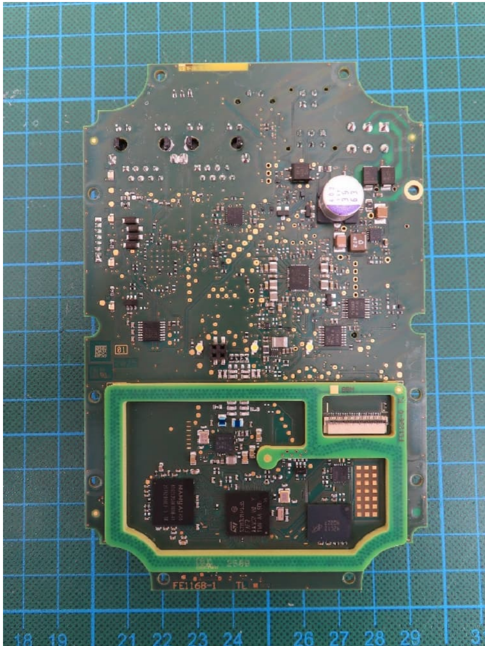
PCB PAY cVEND PIN II – Core PCB, top view
