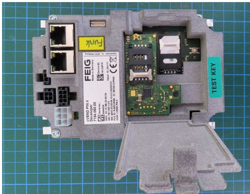
EUT with LTE Modem Extension Board
