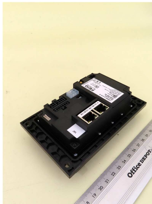
EUT, 3D view 2
