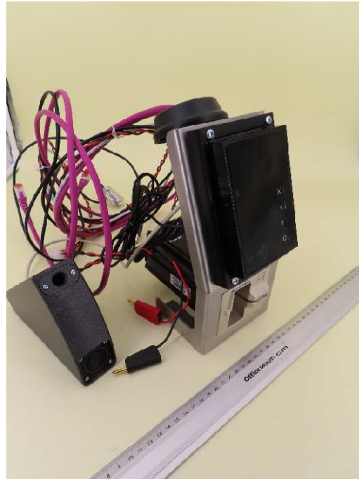
EUT with ancillary, view 1
