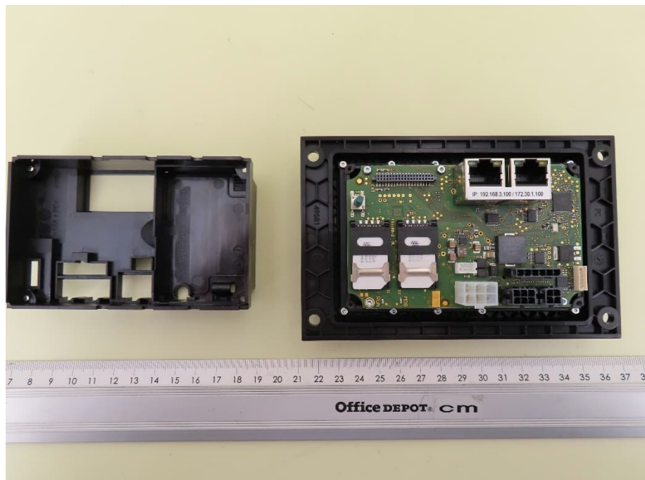
EUT, cover removed, view 1
