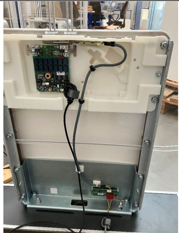
Photo of EUT: ID ANT1710/690-A + ID ANT1710/690-B Configuration: Modul ID LRM5400 (inside ID ANT1710690-A)
