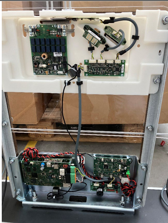
Photo of EUT: ID ANT1710/690-A + ID ANT1710/690-B Configuration: Modul ID LRM5400 (inside ID ANT1710690-A)
