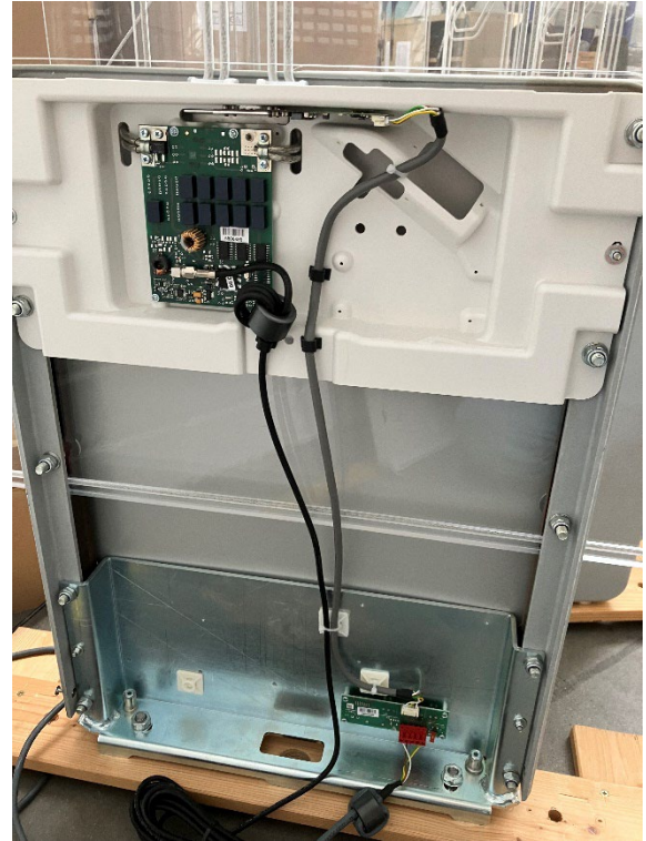
Photo of EUT: ID ANT1520/680-A + ID ANT1520/680-B Configuration: Modul ID LRM5400 (inside ID ANT1520680-A)
