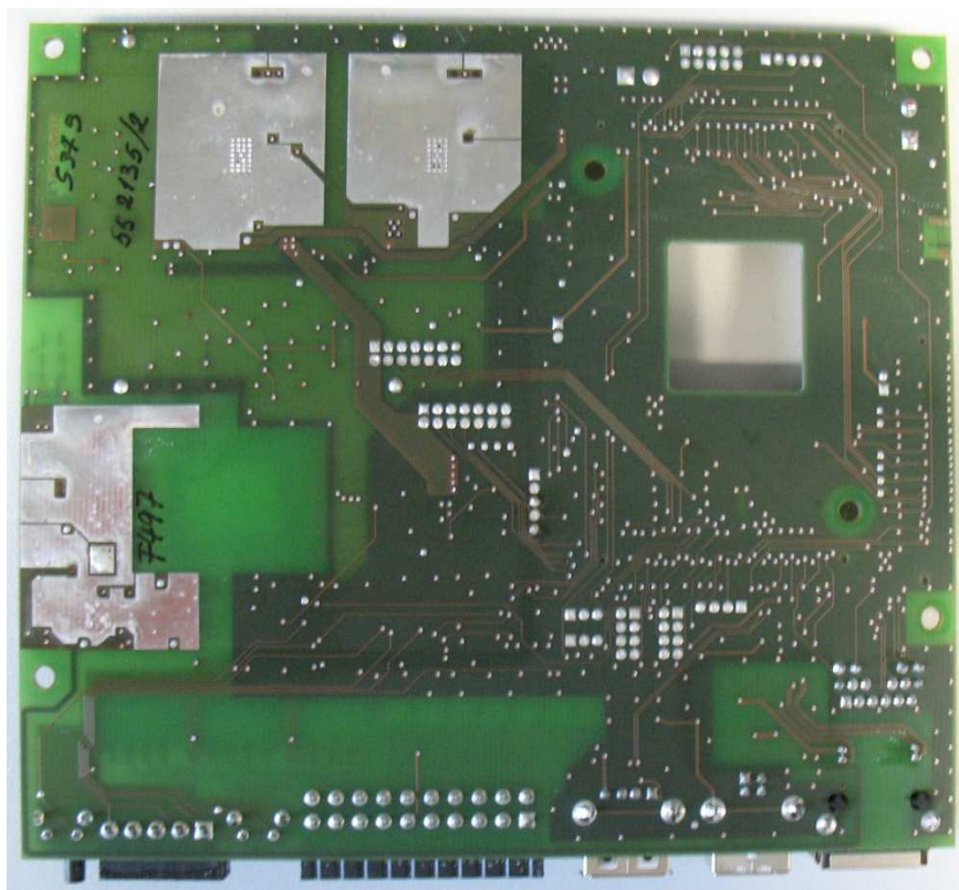
Digital Board – bottom view:
