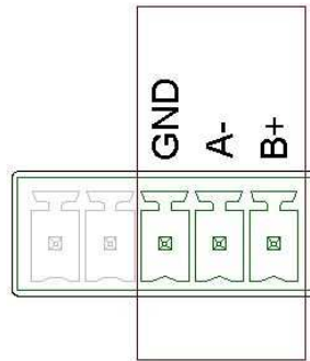
Fig. 10: RS485 interface pin-outs on X6 (RS485-Interface)
