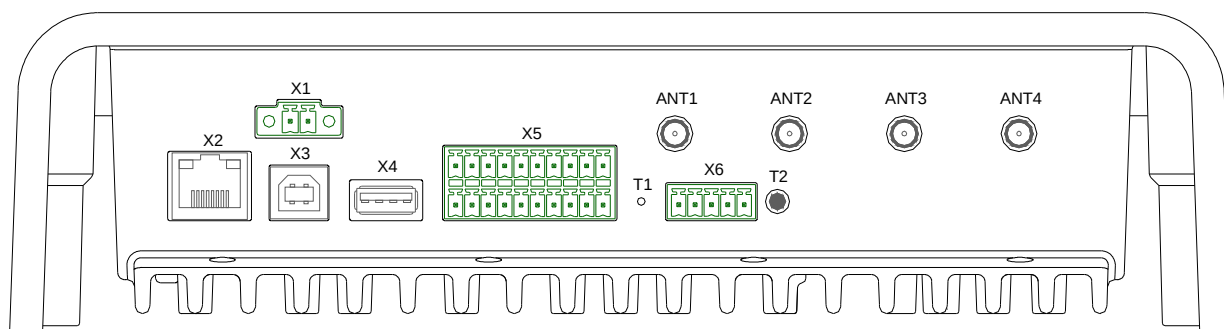
Fig. 2: Connection Overview
