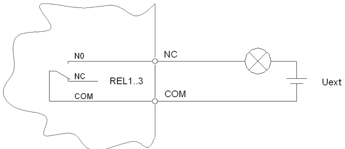
Fig. 18: Internal and external wiring of the relay output
