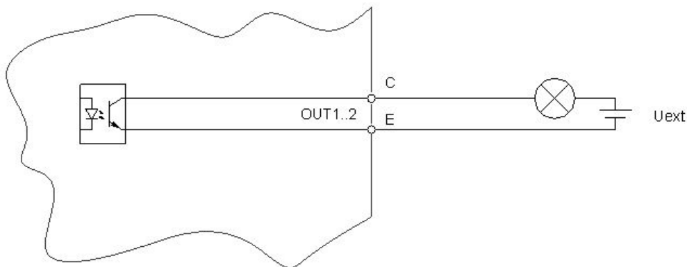
Fig. 16: Internal and external wiring of the optocoupler-outputs OUT1-2
