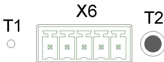
Fig. 19: Position of the reset-switches T1 and T2
