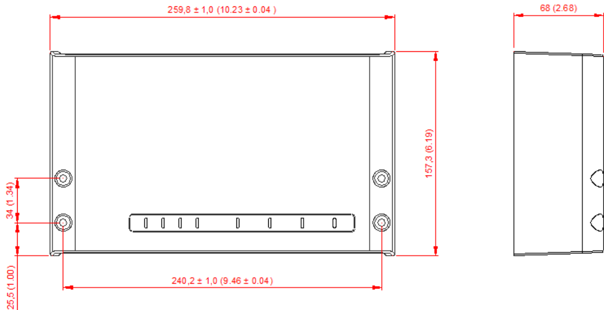
Fig. 1: Installation Drawing
