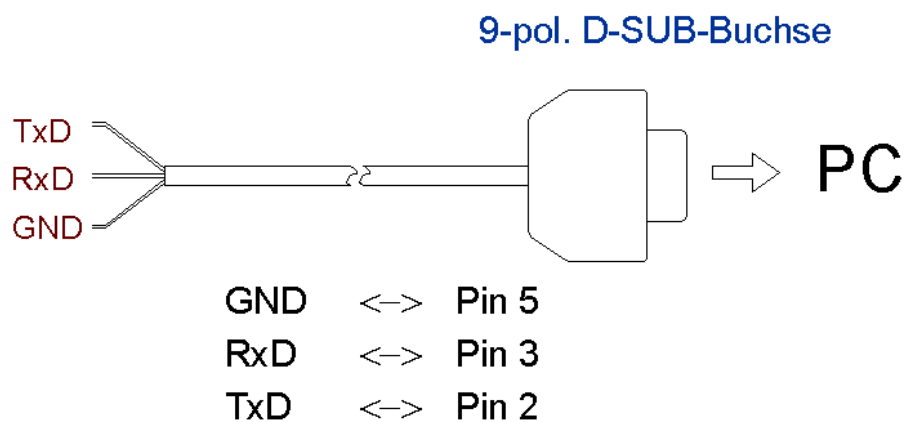
Fig. 9: Wiring example for connecting the RS232 interface X6
