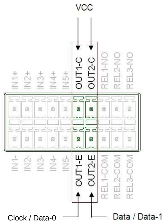
Fig. 11: Data-Clock Interface on connector X5
