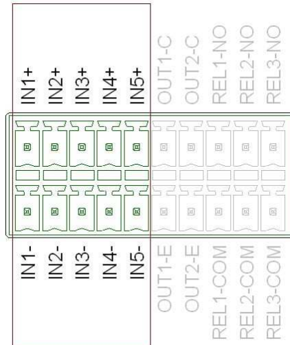
Fig. 13: Optocoupler pin-outs IN1 – IN5
