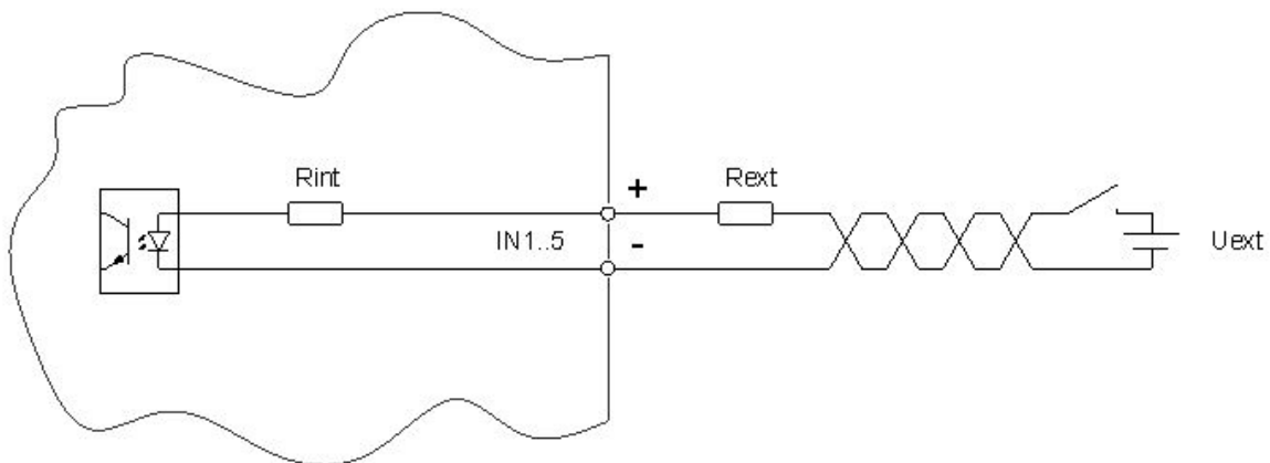
Fig. 14: Internal and possible external wiring of the optocoupler inputs
