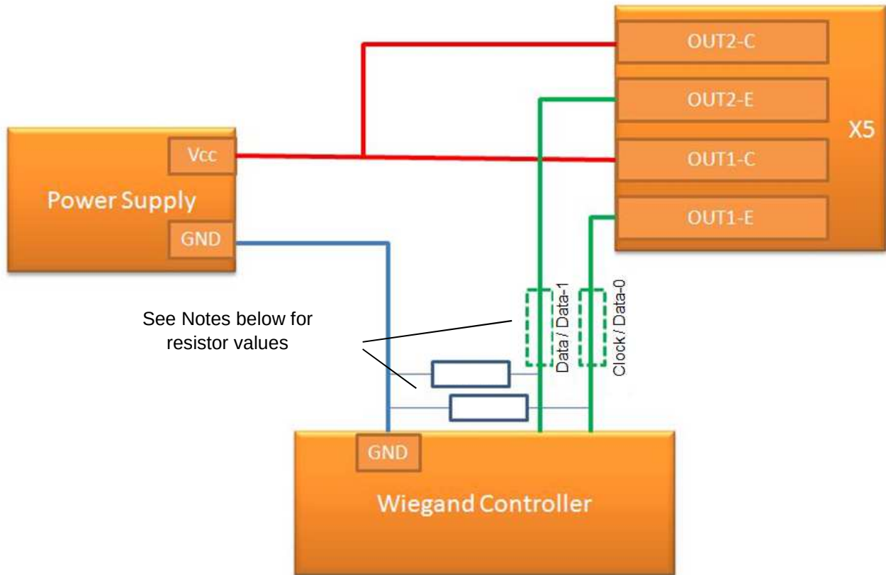
Fig. 12: Wiring Example
