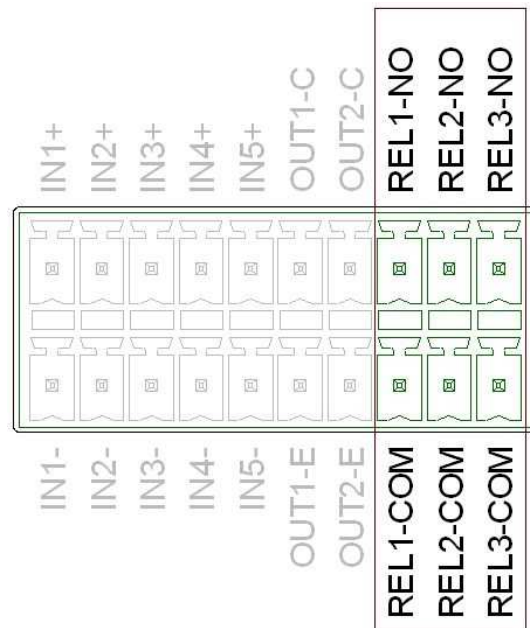
Fig. 17: Relay output pin-outs REL1-3
