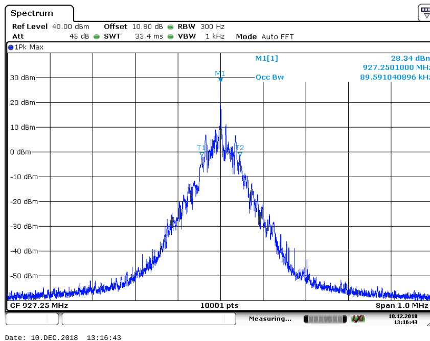
Plot 6: High Channel OBW 99
