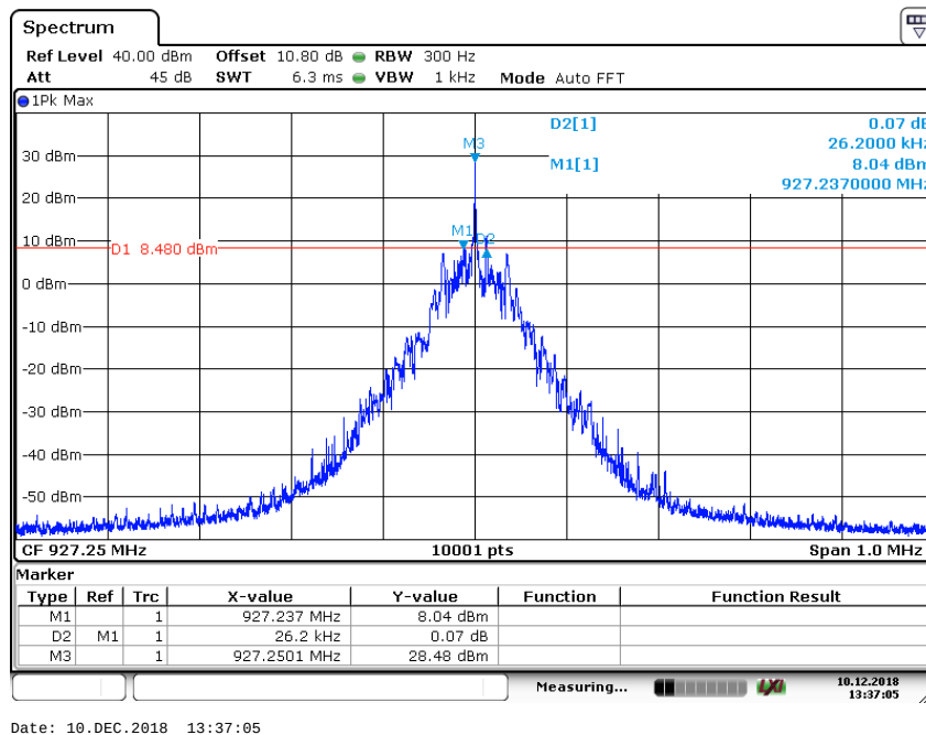
Plot 5: High Channel 20 dB-Bandwidth
