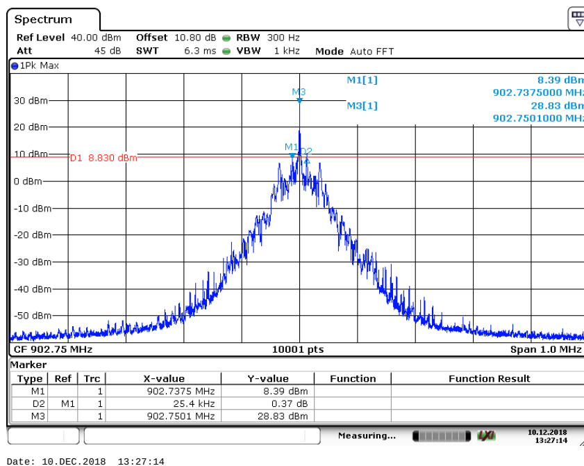
Plot 1: Low Channel 20 dB-Bandwidth
