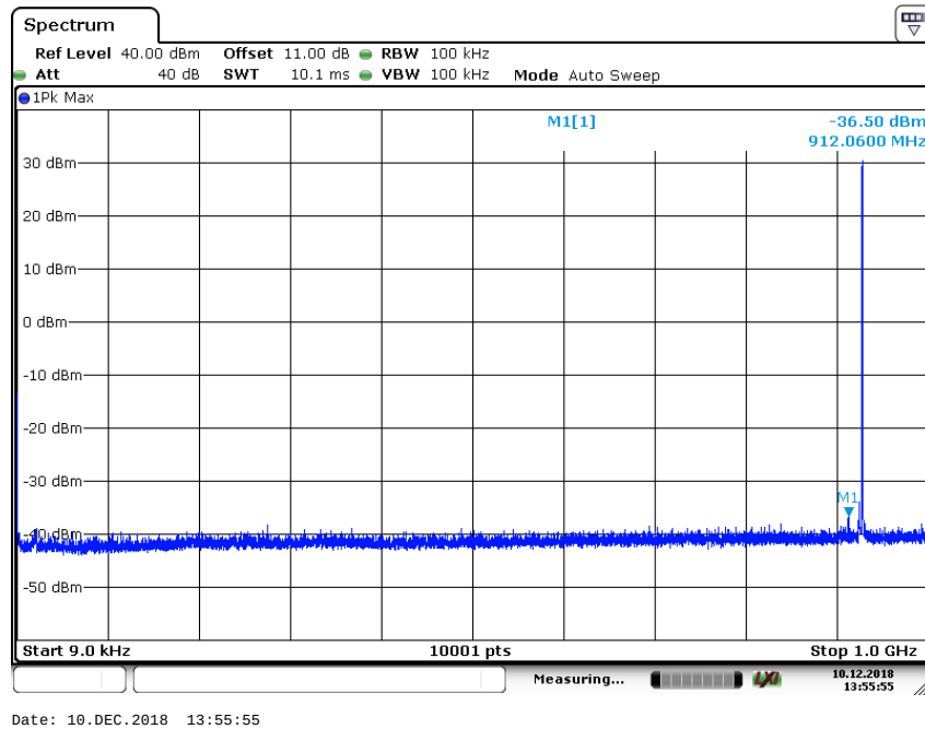
Plot 5: High channel, 9 kHz – 1 GHz
