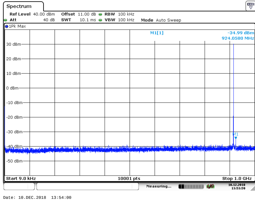
Plot 3: Middle channel, 9 kHz – 1 GHz
