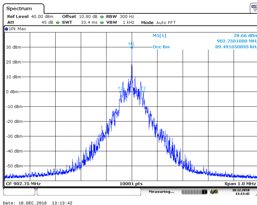
Plot 2: Low Channel OBW 99
