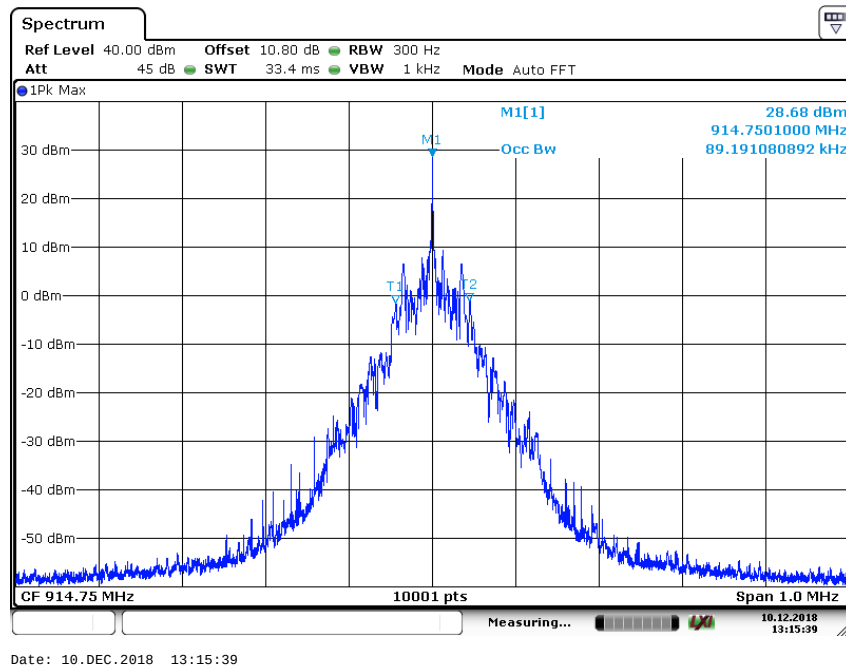
Plot 4: Mid Channel OBW 99
