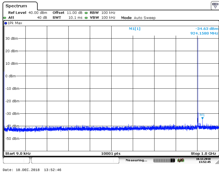
Plot 1: Low channel, 9 kHz – 1 GHz
