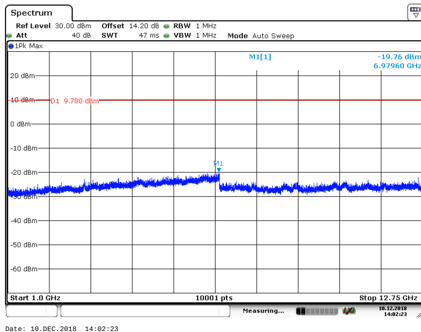
Plot 6: High channel, 1 GHz – 12.75 GHz
