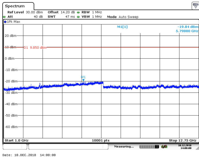
Plot 2: Low channel, 1 GHz – 12.75 GHz
