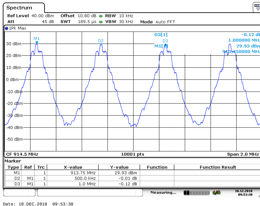
Plot 1: Frequency separation
