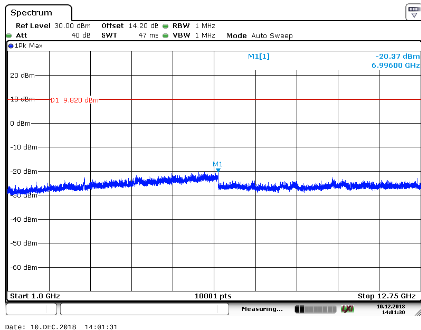
Plot 4: Middle channel, 1 GHz – 12.75 GHz
