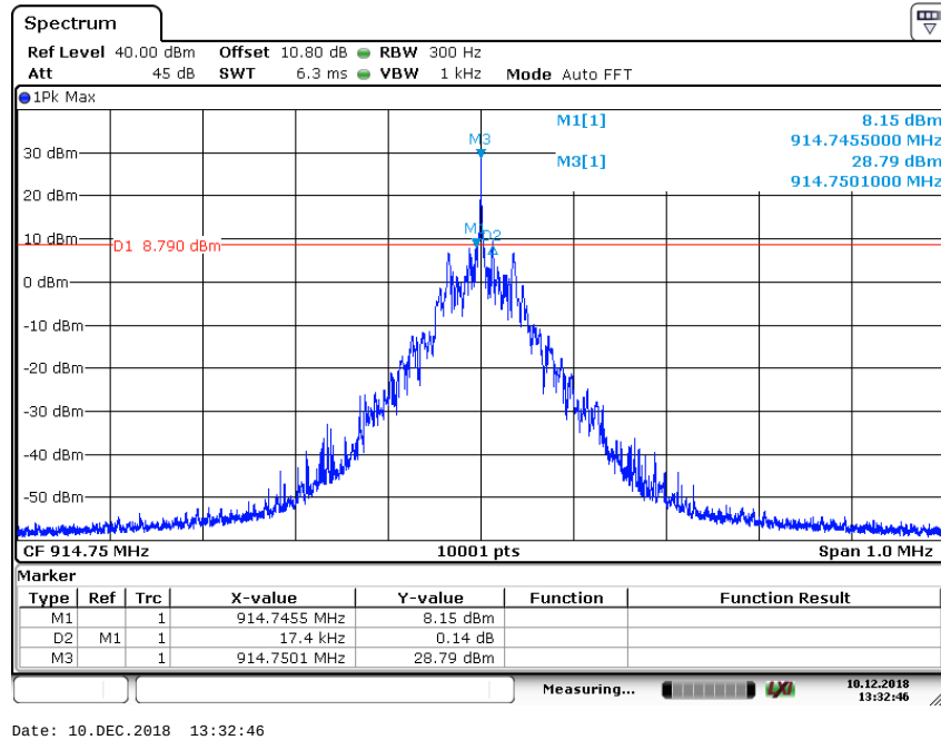
Plot 3: Mid Channel 20 dB-Bandwidth
