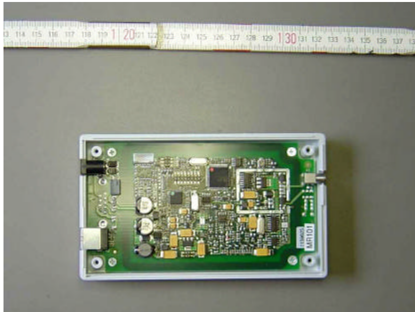
Front of unit
