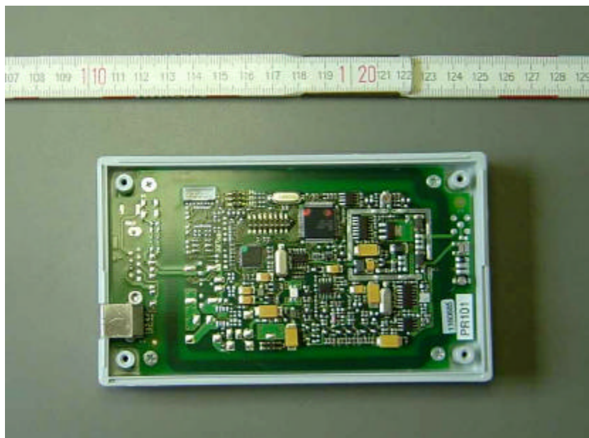
Top view of printed board
