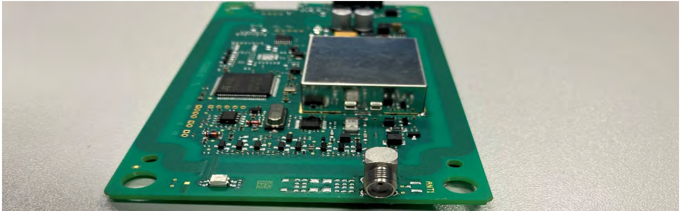
Photo of EUT: Internal construction side view
