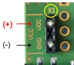
Fig 8: Pin assignment +/-
