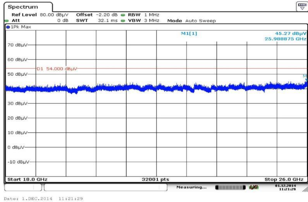
Plot 11: Middle channel; 18 GHz to 26 GHz, horizontal &amp; vertical polarization
