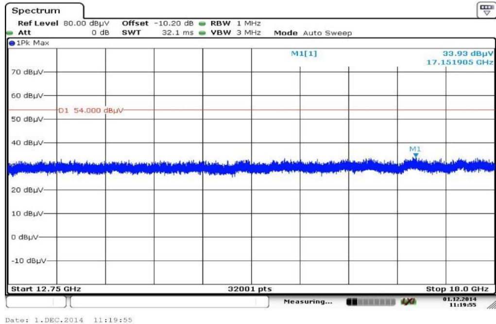
Plot 4: Receiver mode (12.75 GHz – 18 GHz)
