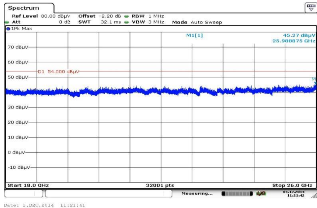
Plot 17: Highest channel; 18 GHz to 26 GHz, horizontal &amp; vertical polarization
