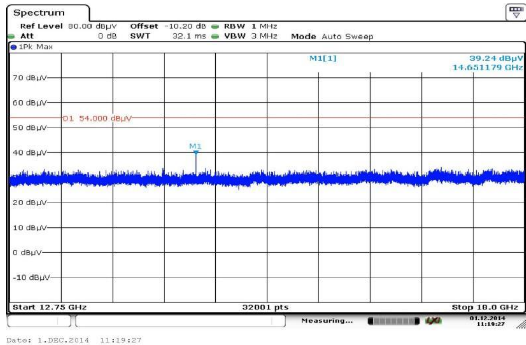
Plot 16: Highest channel; 12 GHz to 18 GHz, horizontal &amp; vertical polarization
