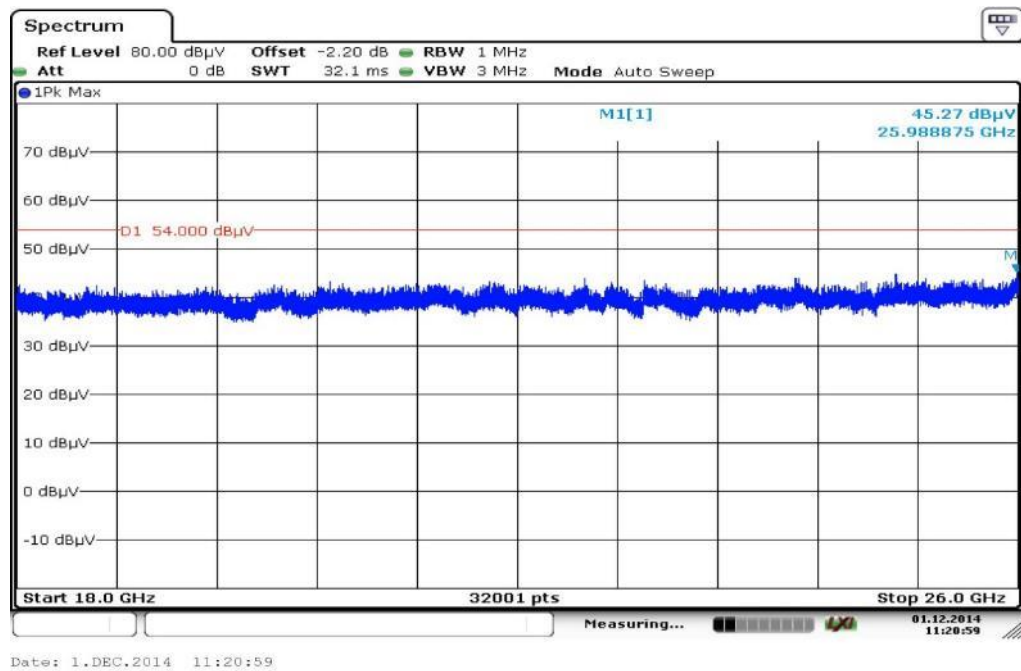
Plot 6: Lowest channel; 18 GHz to 26 GHz, horizontal & vertical polarization
