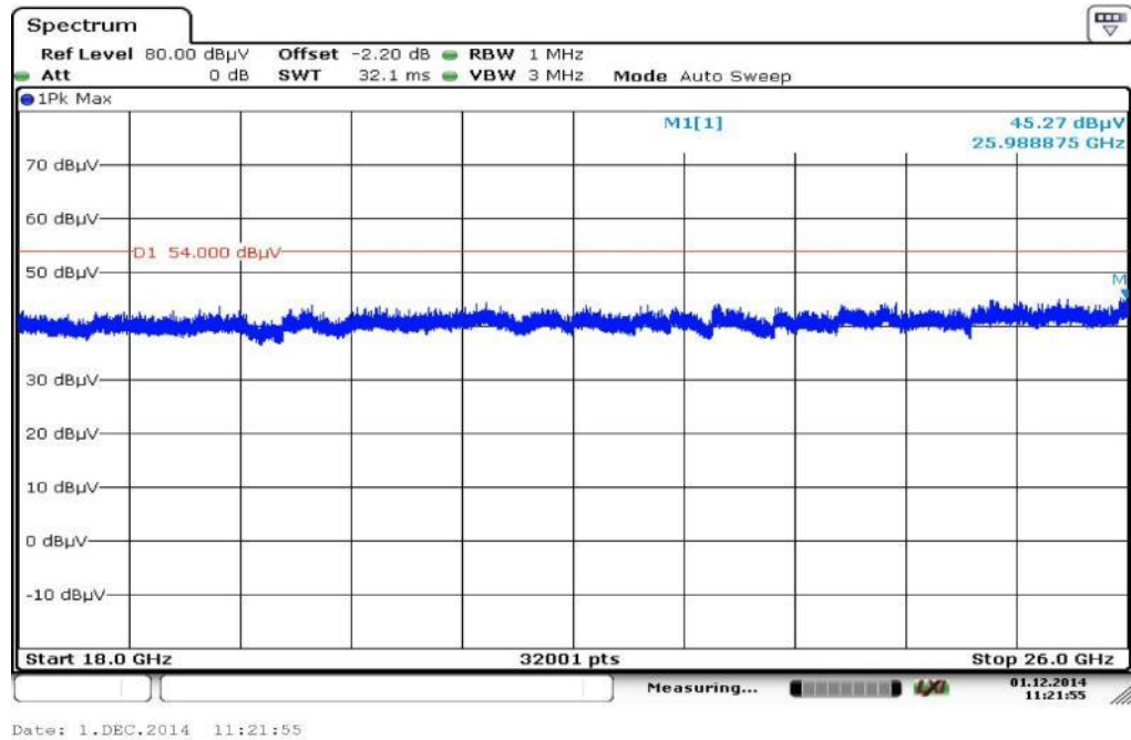
Plot 5: Receiver mode (18 GHz – 26 GHz)
