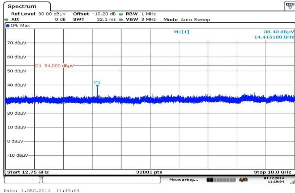
Plot 10: Middle channel; 12 GHz to 18 GHz, horizontal &amp; vertical polarization
