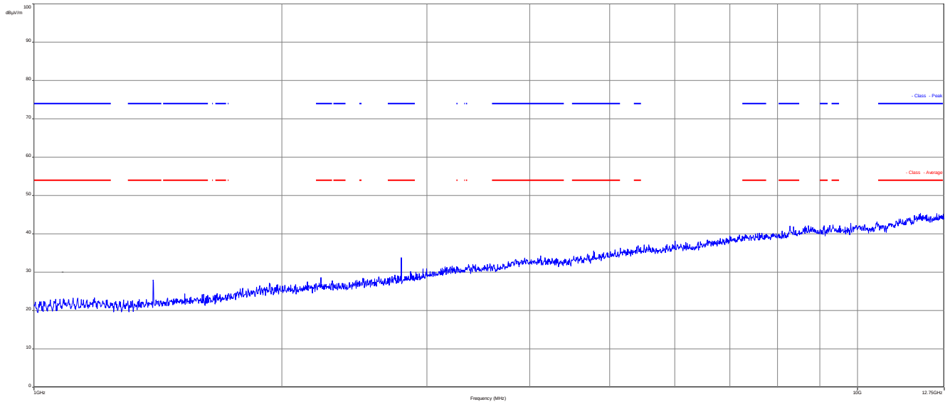
Plot 3: Receiver mode (1 GHz – 12.75 GHz)
