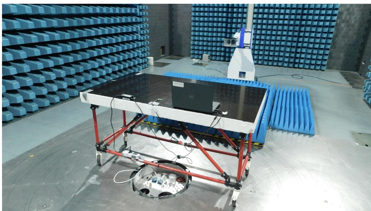
Picture 4: EUT test setup radiated emission test > 1 GHz (rear view)
