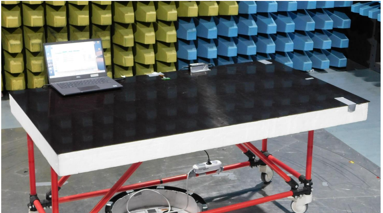
Picture 1: EUT test setup radiated emission test < 1 GHz (front view)
