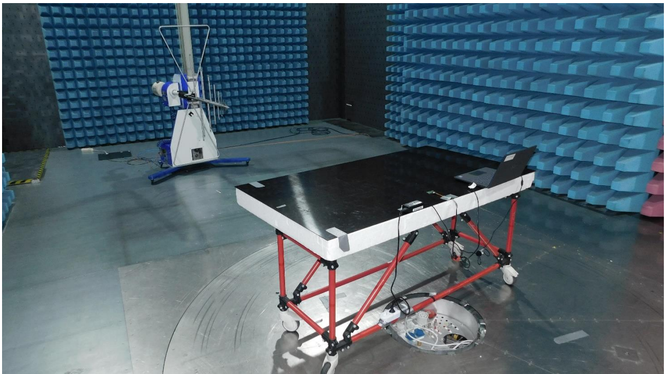
Picture 2: EUT test setup radiated emission test < 1 GHz (rear view)
