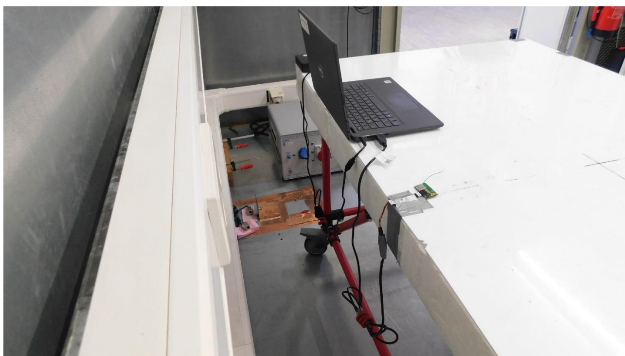
Picture 6: EUT test setup conducted emission test (rear view)
