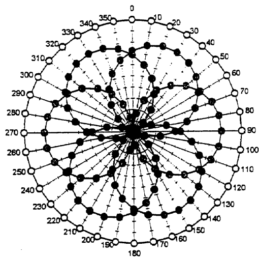
f = 2500 \text{ MHz, WG R26}
